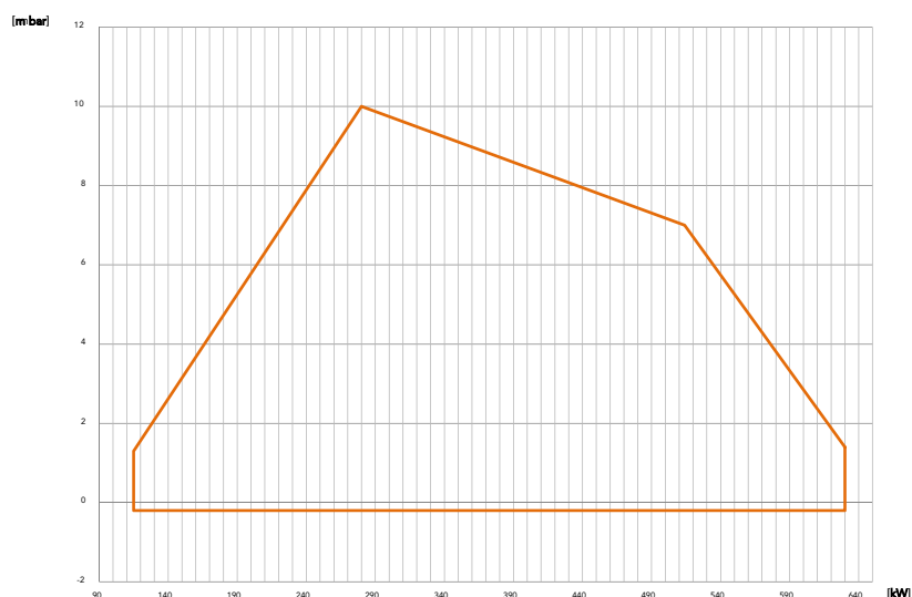
Fig. 2 X = Thermal power Y = Pression in the combustion chamber
