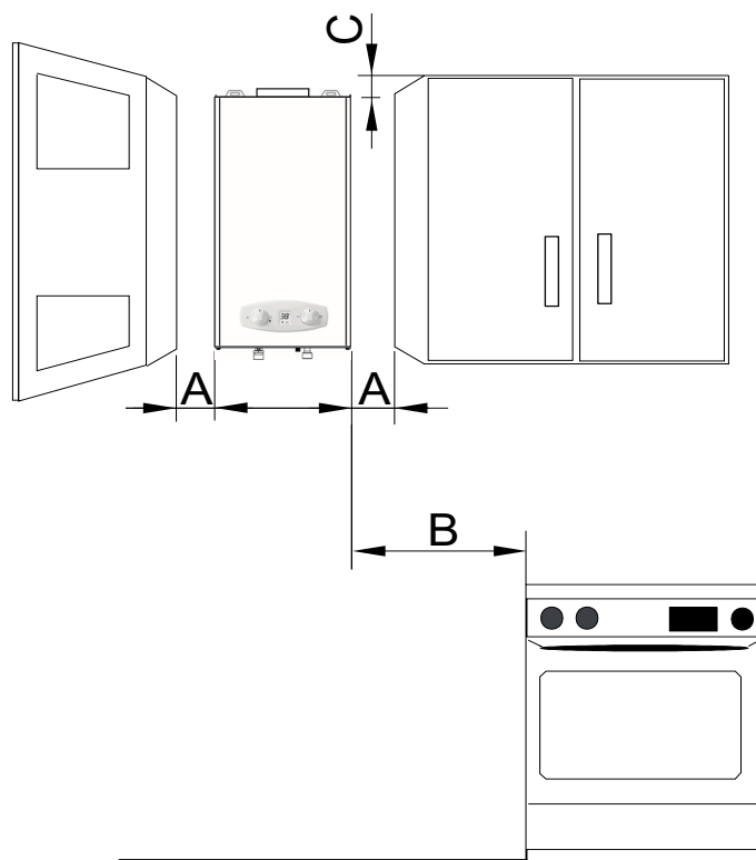
fig. 5 - Minimum distances
