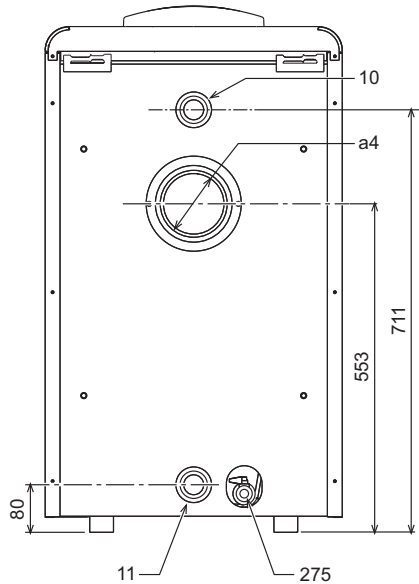
fig. 25 - Dimensions, connections and main components
