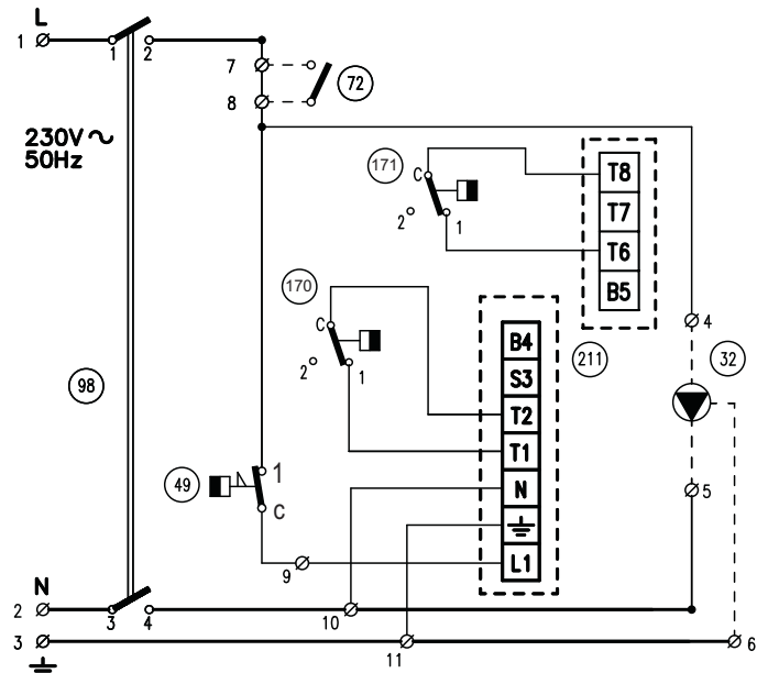
fig. 29 - Main wiring diagram G3G 80 - 98
