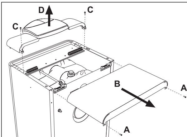
fig. 24 - Accessing the terminal block
