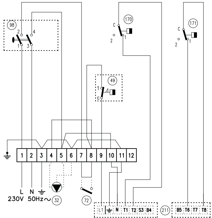
fig. 30 - Electrical connection diagram G3G 80 - 98
