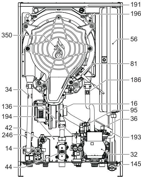
fig. 62- General view
