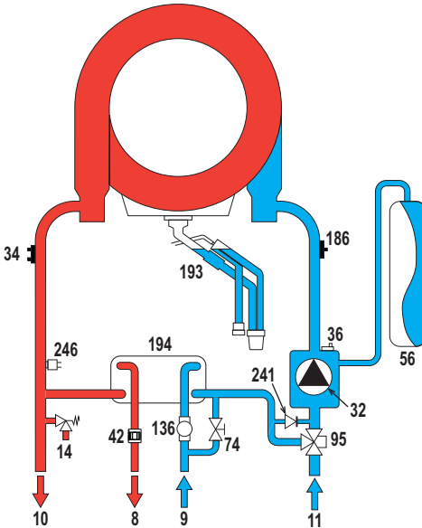
fig. 63- Hydraulic circuit
