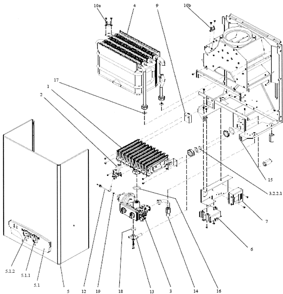
Rys. A Ogrzewacz AcquaProJet 11 i Draw. A Gas water heater AcquaProJet 11 i Zeich. A Gaswasserheizer AcquaProJet 11 i
