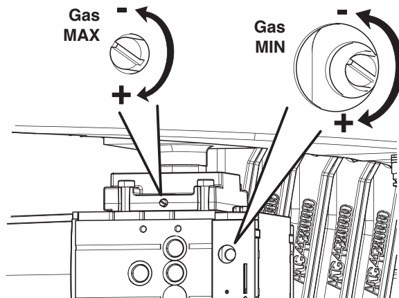
Valvola gas POWERCOND 200 / 240 / 280
