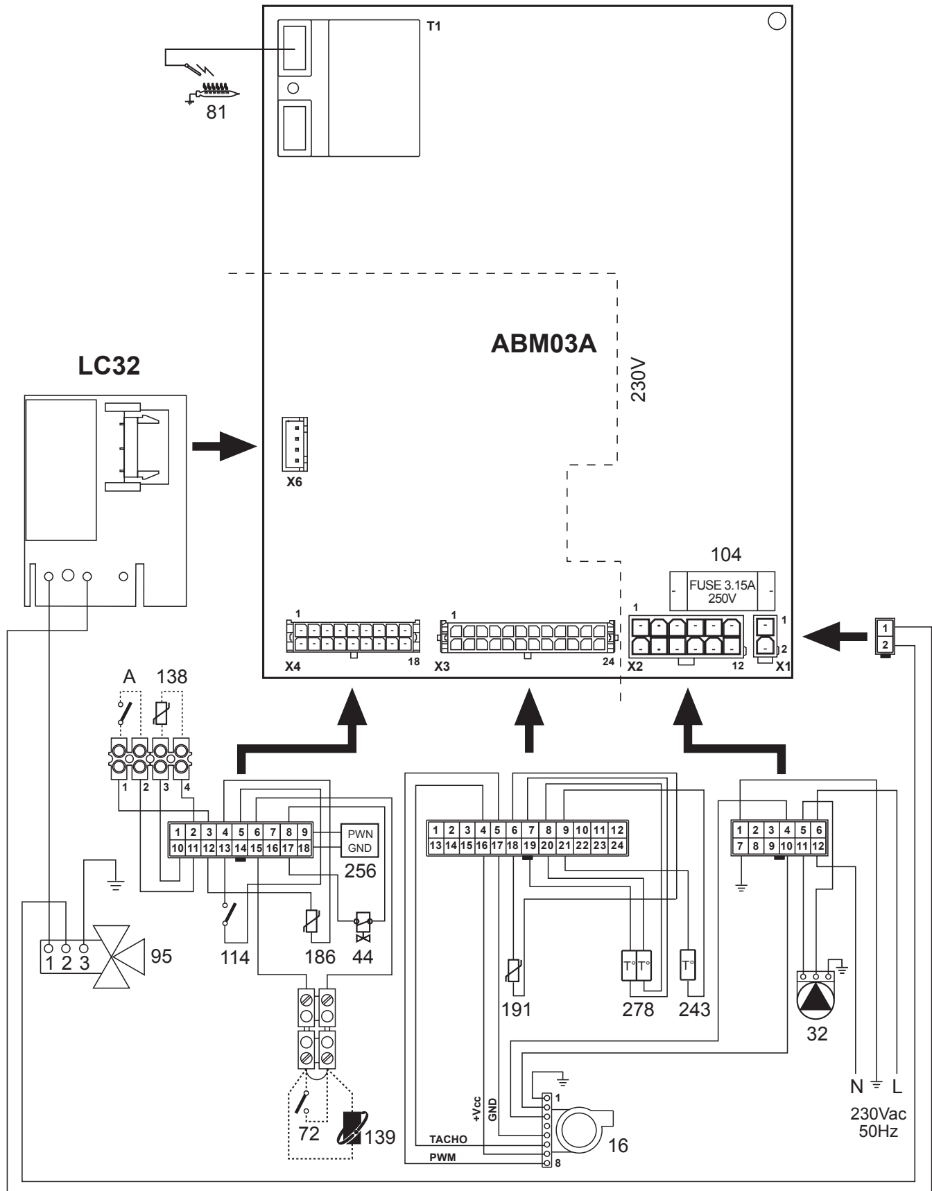
fig. 29 - Wiring diagram
