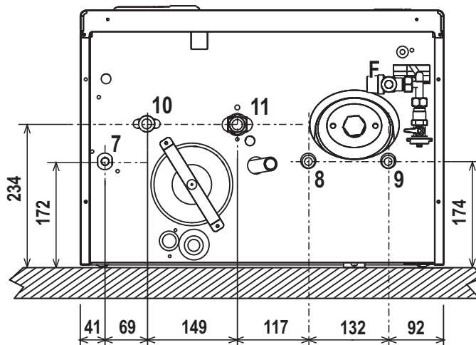
fig. 13 - Plumbing connections
