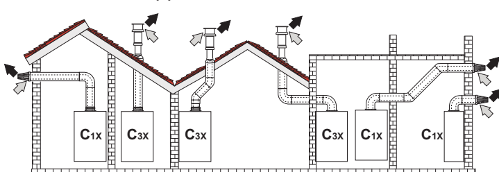
fig. 15 - Examples of connection with coaxial pipes (⇨ = Air / ⇨ = Fumes)
