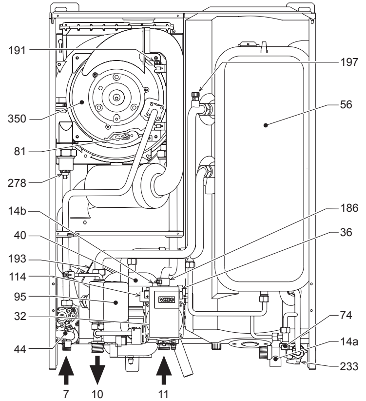
fig. 26 - Front view
