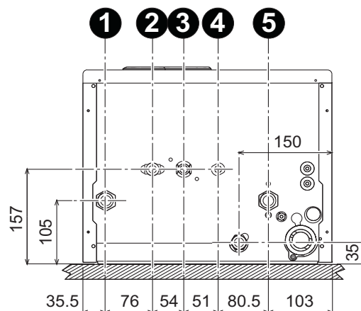
fig. 13 - Raccordements hydrauliques
