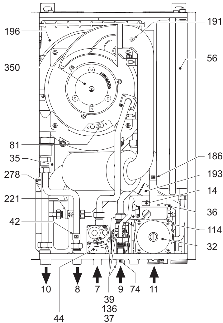
fig. 26 - General view
