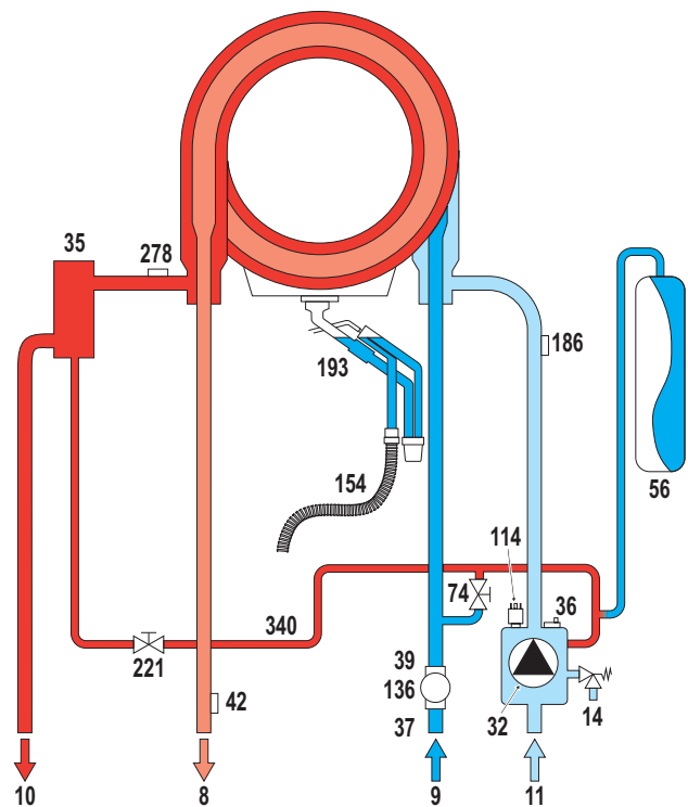
fig. 27 - Water circuit
