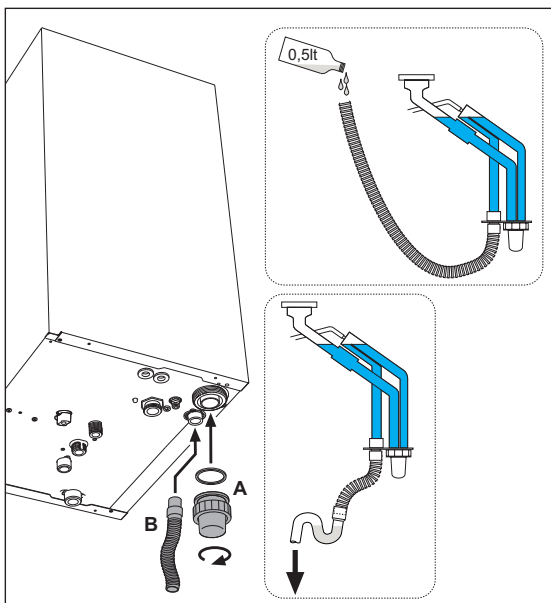
fig. 20 - Condensate outlet connection
