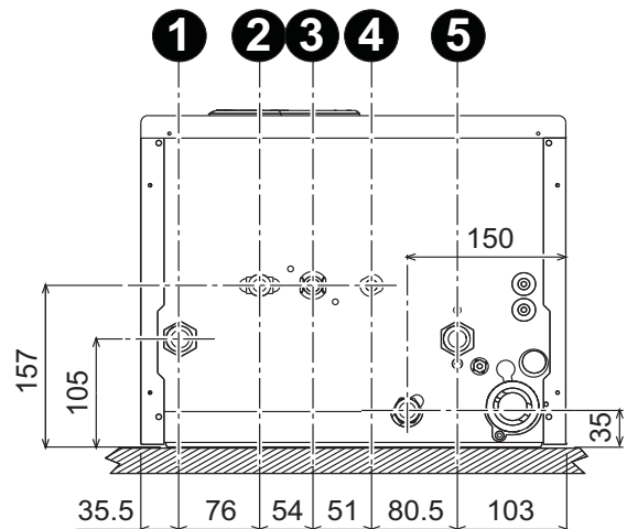
fig. 13 - Plumbing connections
