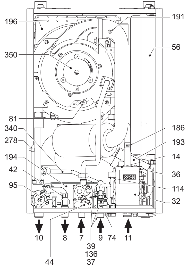
fig. 26 - General view
