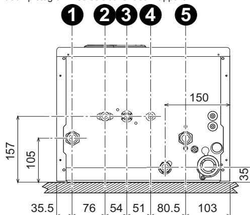
fig. 13 - Raccordements hydrauliques
