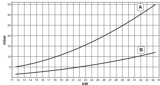
fig. 23 - Pressure - power diagram (DOMItech F 32 D)
