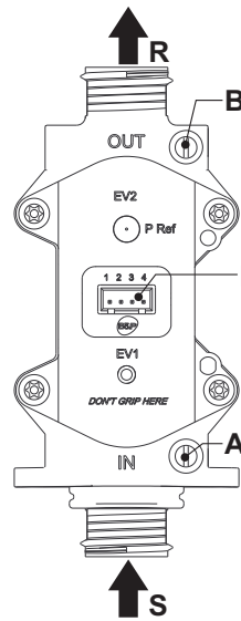
fig. 15 - Gas valve
