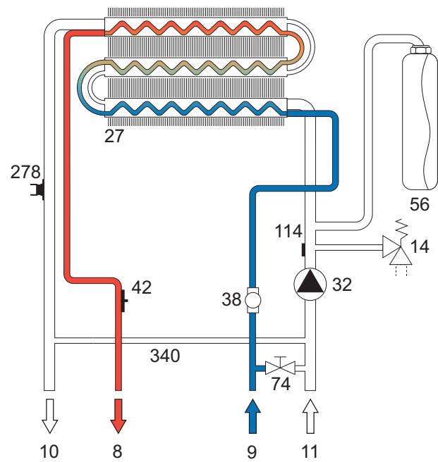
fig. 21 - DHW Circuit
