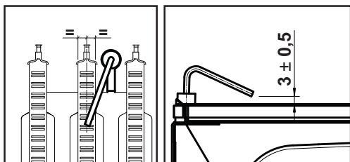
fig. 17 - Electrode positioning
