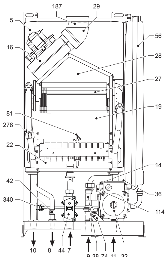
fig. 18 - Vista general DOMItech F 24 D
