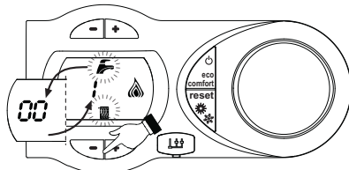
fig. 14 - TEST mode (heating power = 100%)
