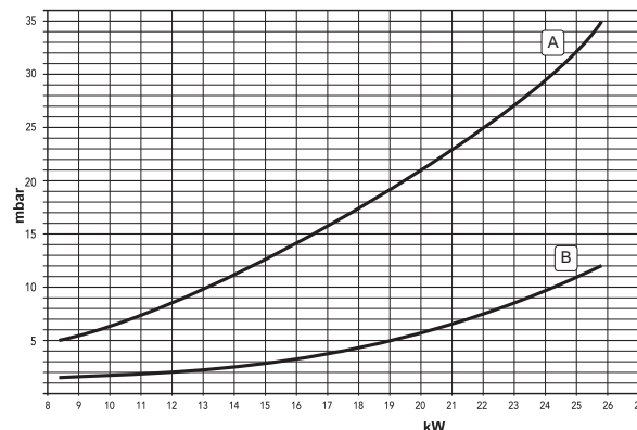
fig. 22 - Pressure - power diagram (DOMItech F 24 D)
