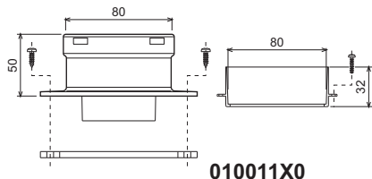
fig. 12 - Starting accessory for separate ducts
