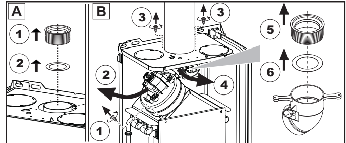
A Baffle replacement with boiler not installed B Baffle replacement with boiler and fume ducts already installed
