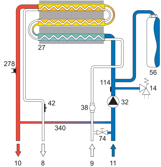
fig. 20 - Heating Circuit
