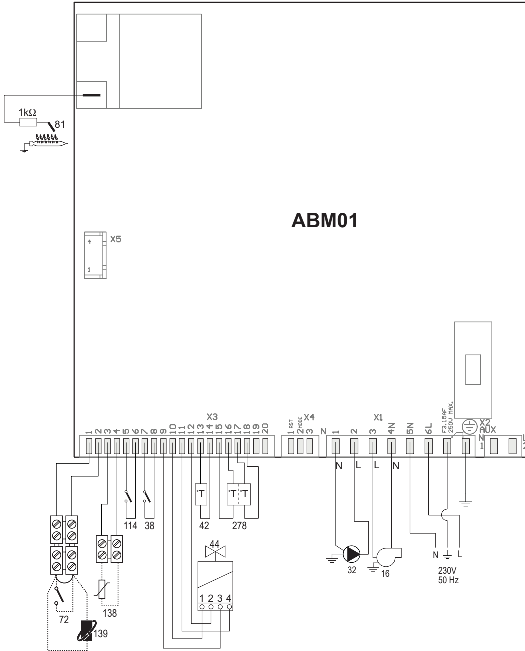
fig. 26 - Electrical circuit
