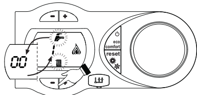
fig. 14 - Mode TEST (puissance chauffage = 100%)
