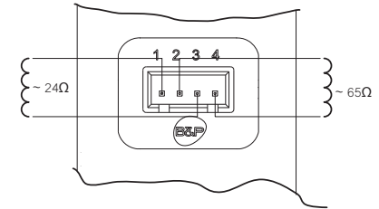
fig. 16 - Gas valve connection
