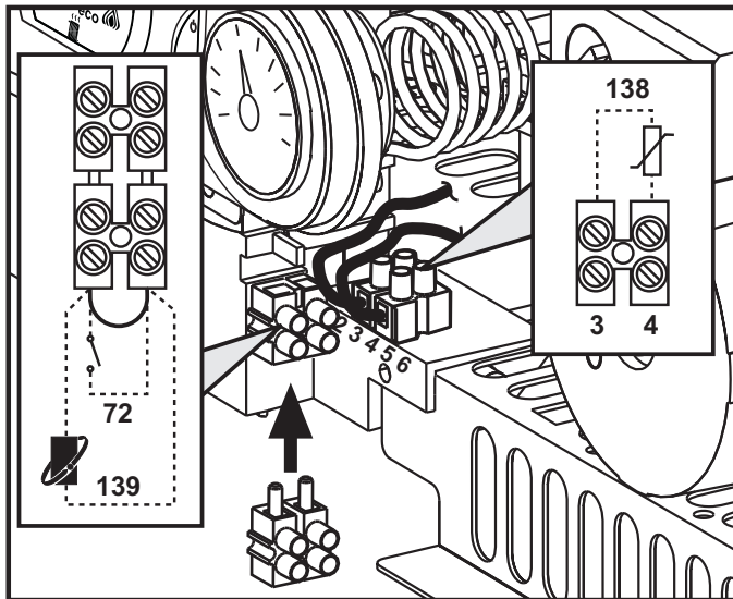
fig. 8 - Accessing the terminal block
