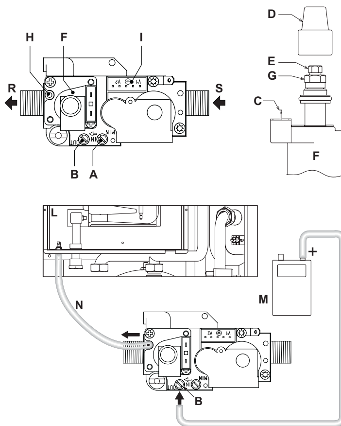
fig. 25 - Valvola gas
