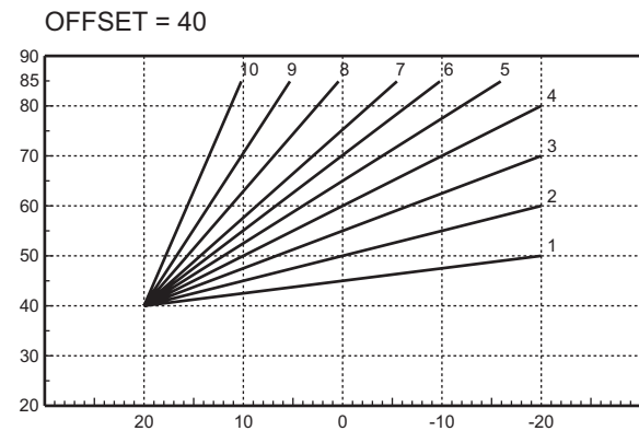
fig. 15 - Example of parallel compensation curve shift
