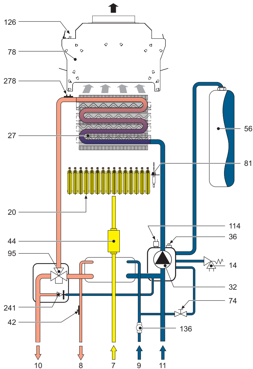
fig. 26 - Plumbing circuit
