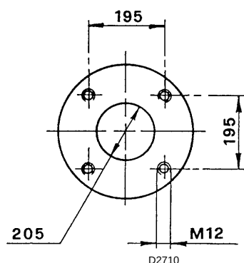
Plaque chaudière
