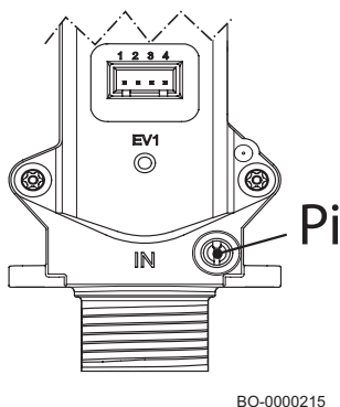
Fig.54 Valvola gas
