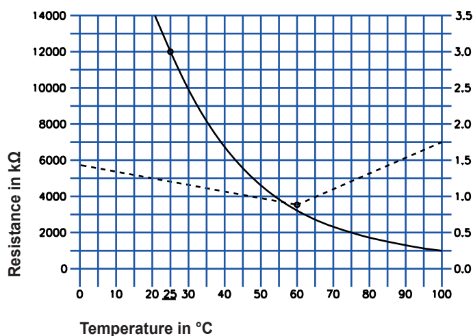
Outlet temperature sensor
