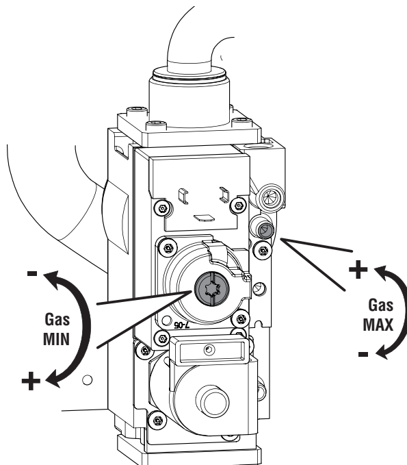
Valvola gas etiKa Power 95 - 110 - 115 - 150
