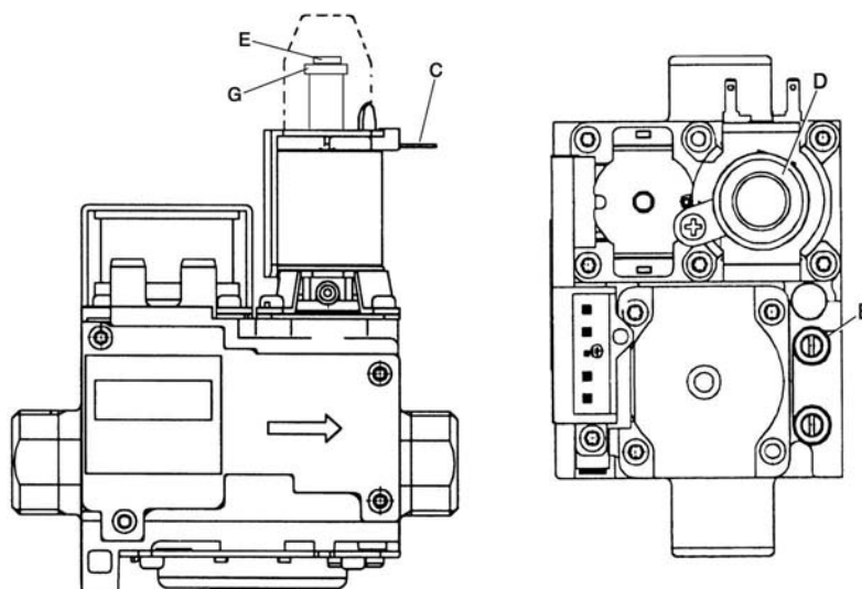
fig. 16 - Valvola gas
