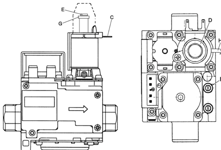
fig. 23 - Valvola gas
