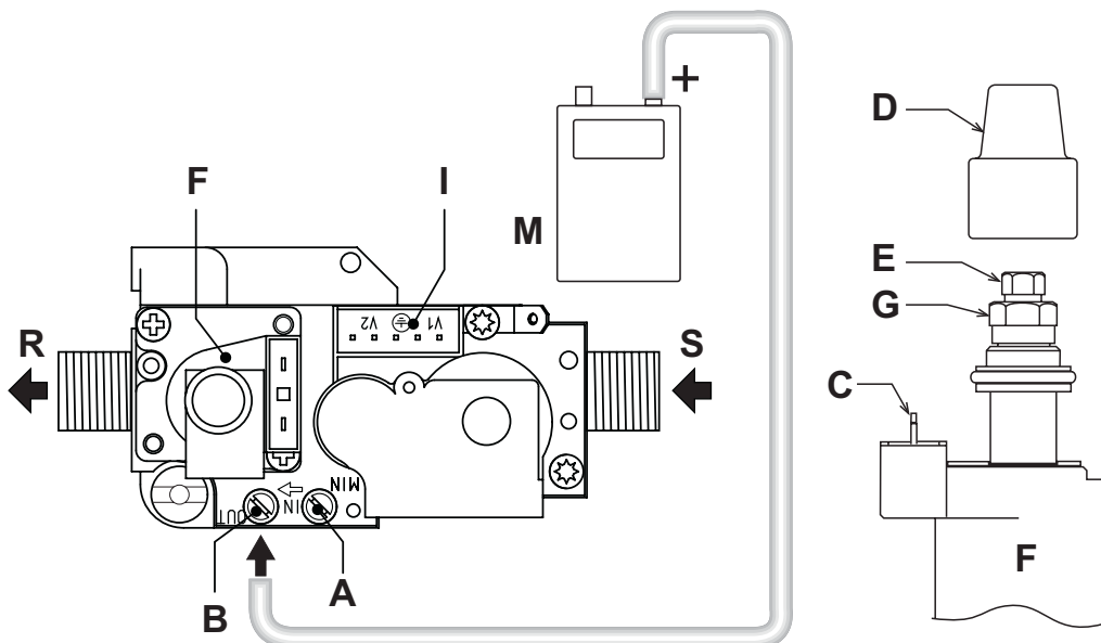
fig. 23 - Valvola gas
