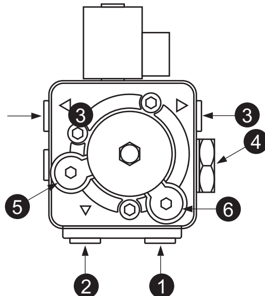
fig. 29- Pump ITALPUMP
