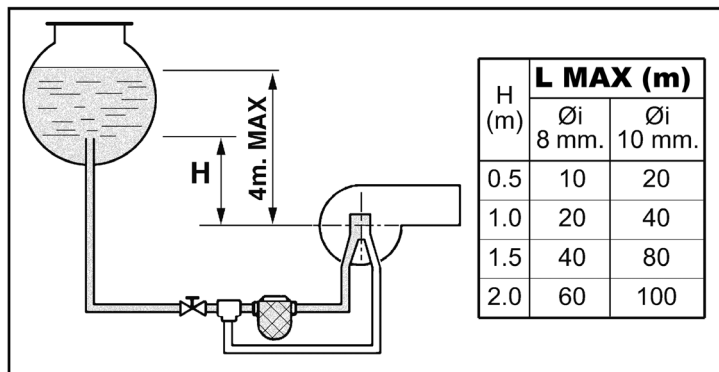
fig. 23 - Gravity feed
