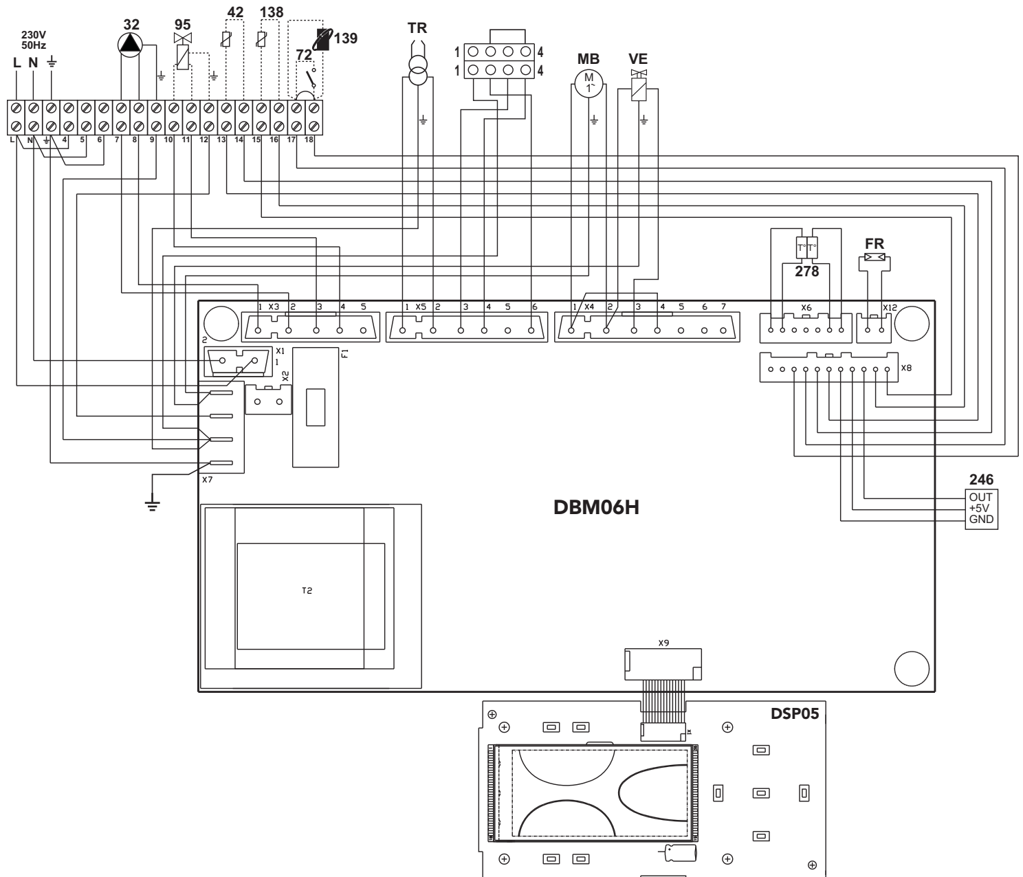
fig. 45 - Wiring diagram
