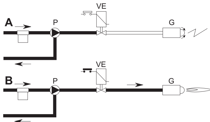
fig. 34 - Starting
