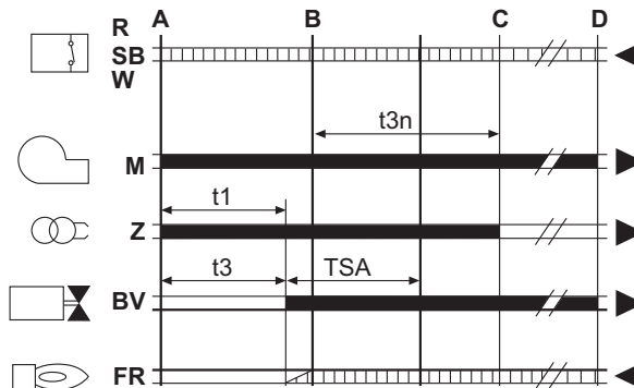
fig. 35 - Unit cycle
