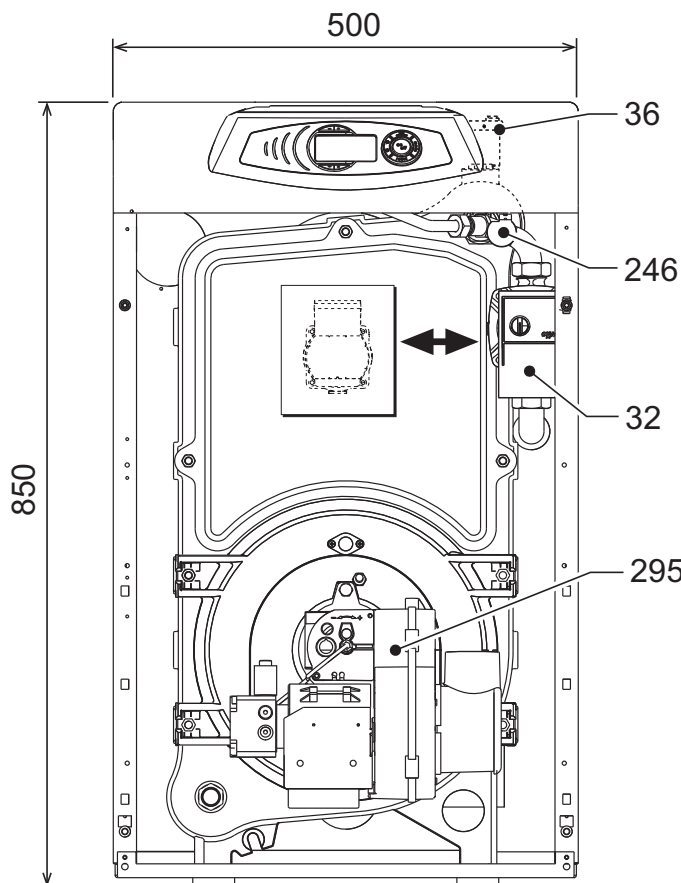
fig. 40- Main components, dimensions and connections
