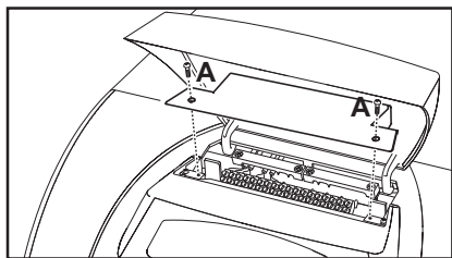
fig. 27 - Accessing the terminal board
