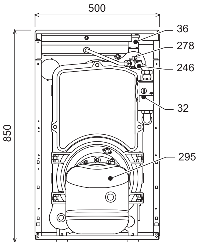
fig. 36 - Dimensions, connections and main components
