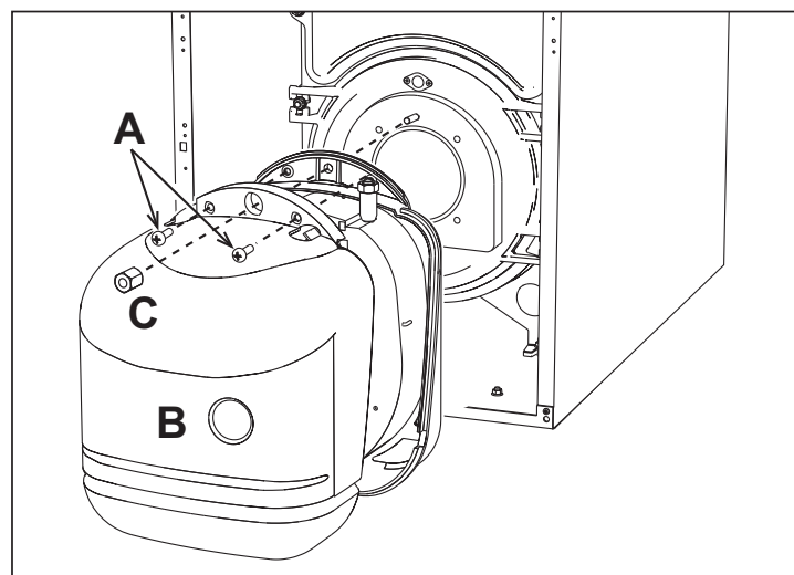
fig. 34 - Burner disassembly
