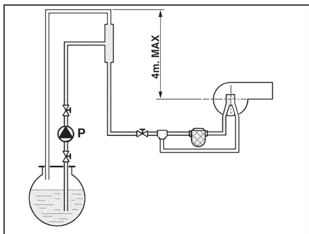
fig. 24 - Ring feed
