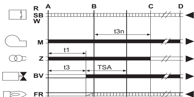
fig. 33 - Unit cycle
