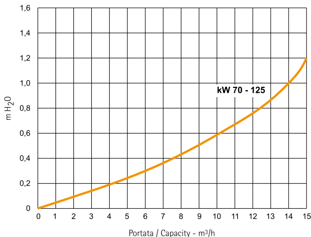
OPERA 70 - 125
