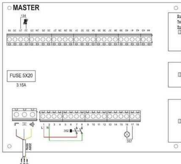
fig. 51- MASTER
