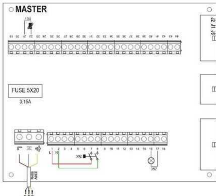
fig. 51- MASTER
