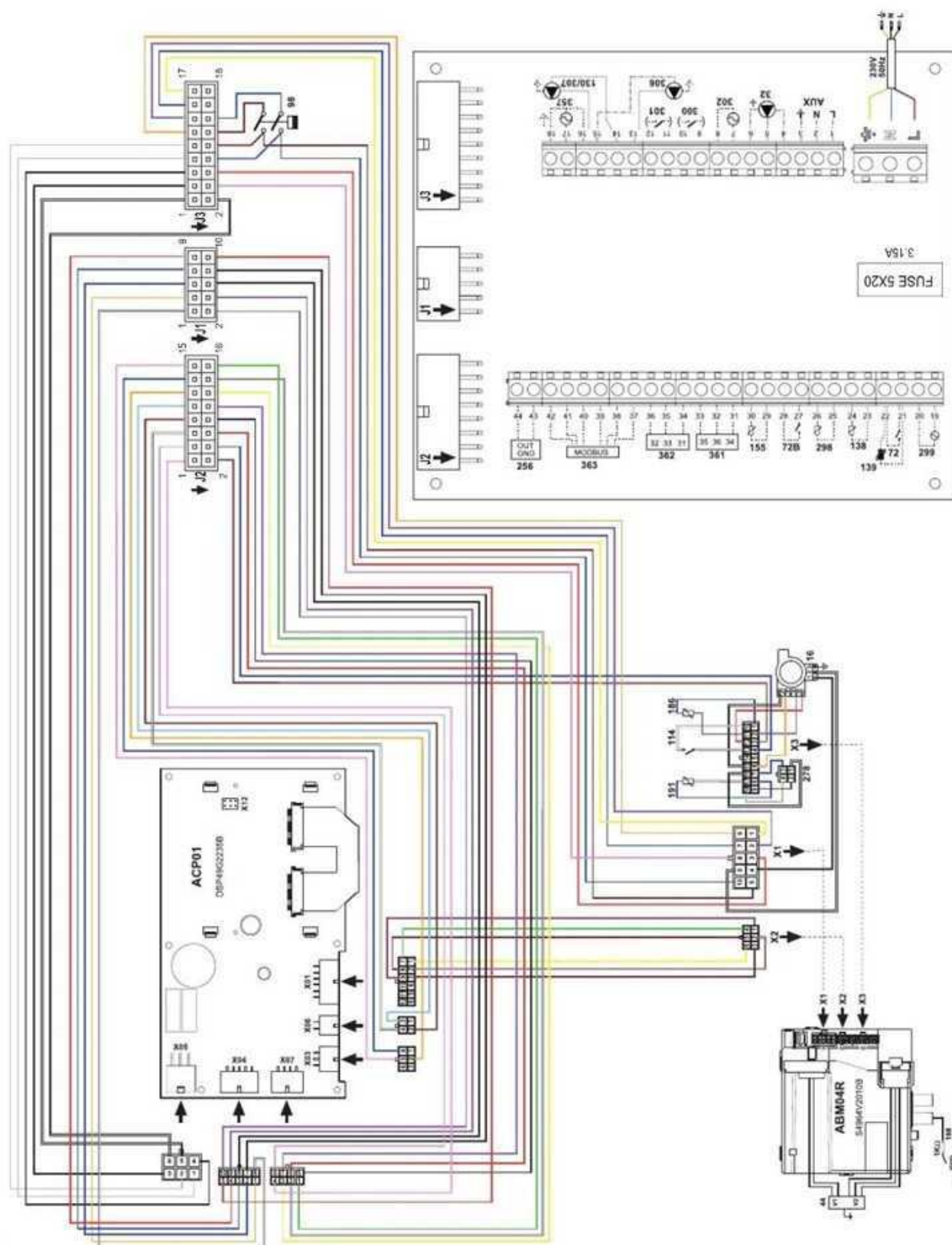
fig. 96- Wiring diagram OPERA 125 and 160
