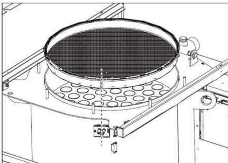
fig. 67 - Alignment of the burner
