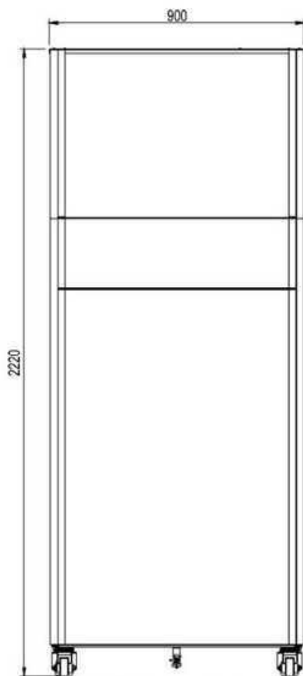
fig. 86- Front view model 450
