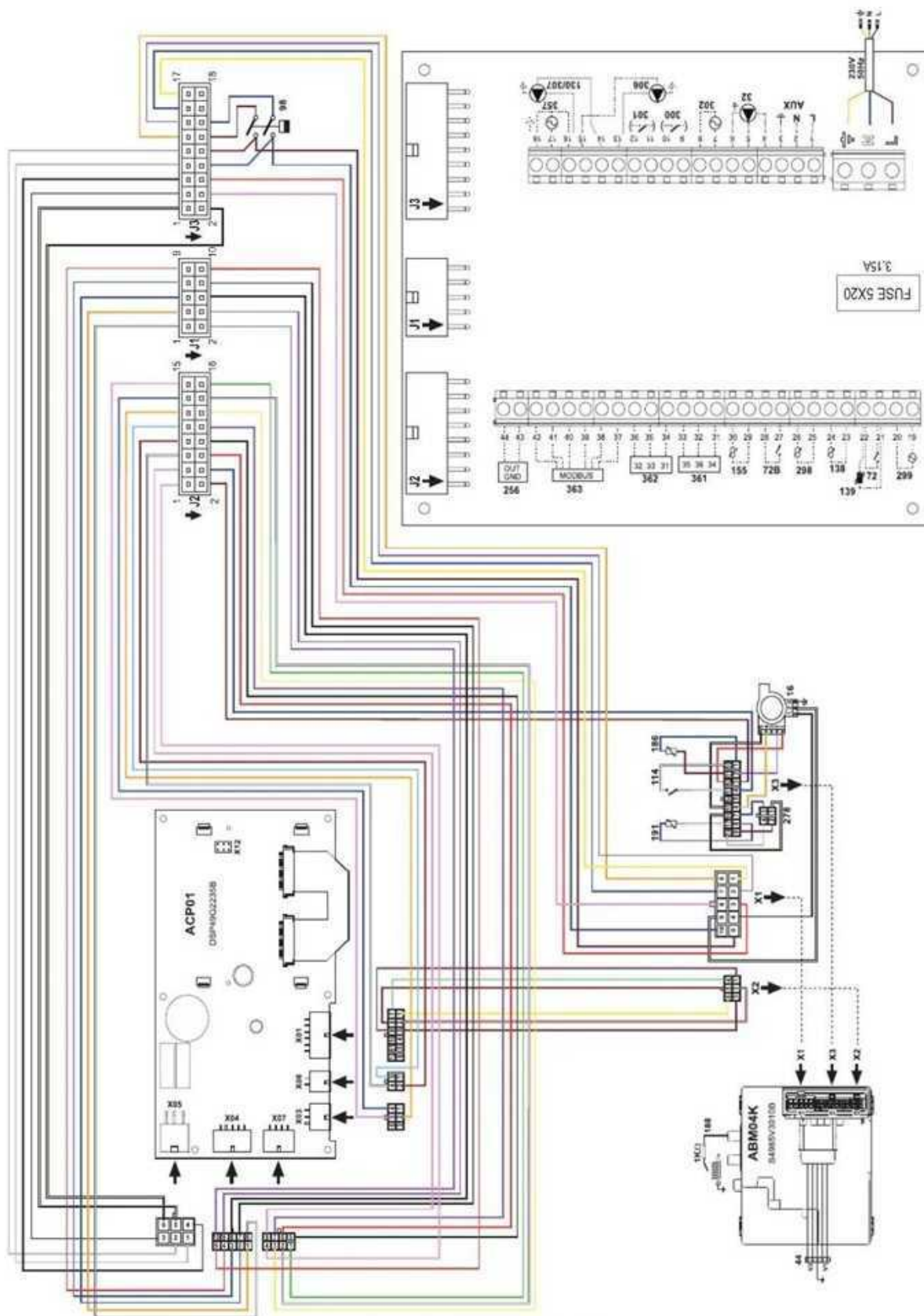
fig. 95- Wiring diagram OPERA 70
