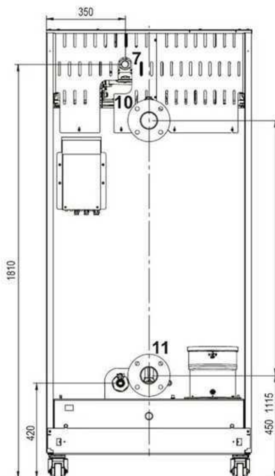
fig. 84- Rear view model 320
