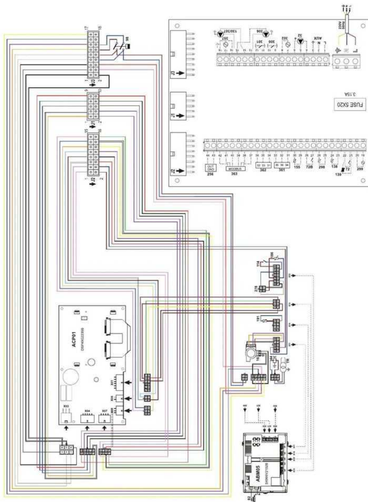
fig. 97- Wiring diagram OPERA 220/320 and OPERA 450
