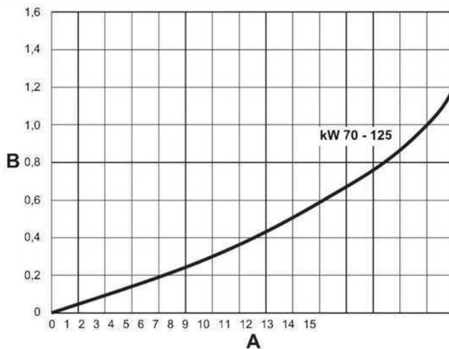
fig. 90 - Pressure loss diagram models 70 - 125
