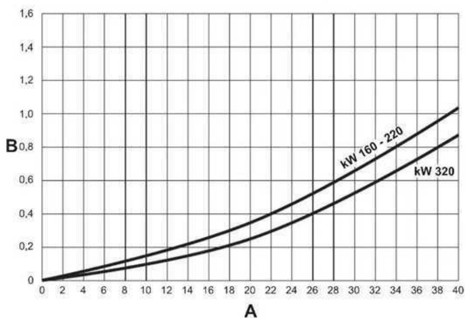
fig. 91 - Pressure loss diagram models 220, 320 and 450
