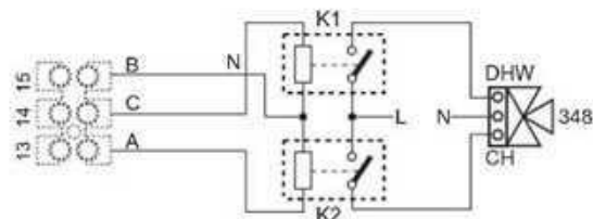
fig. 93- Connection of the 3-way valve with 3 wires
