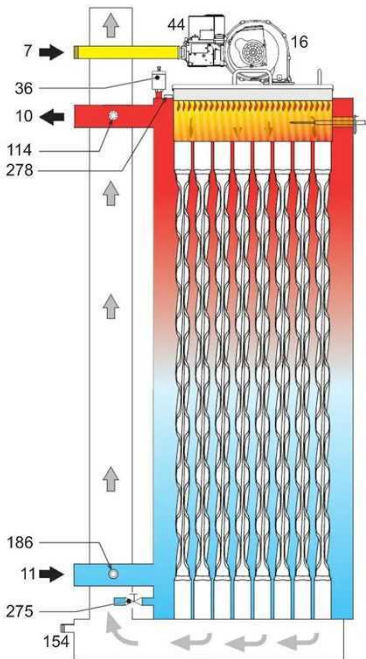
fig. 89- Hydraulic circuit
