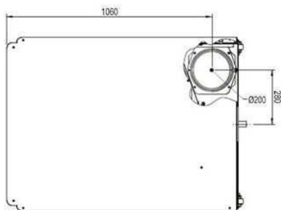
fig. 85- Top view model 320
