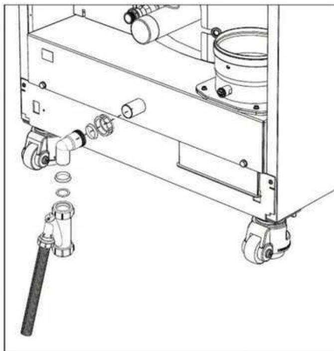
fig. 58- Condensate drain connection
