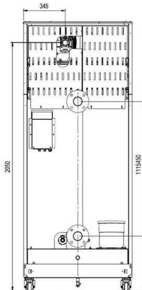
fig. 87- Rear view model 450
