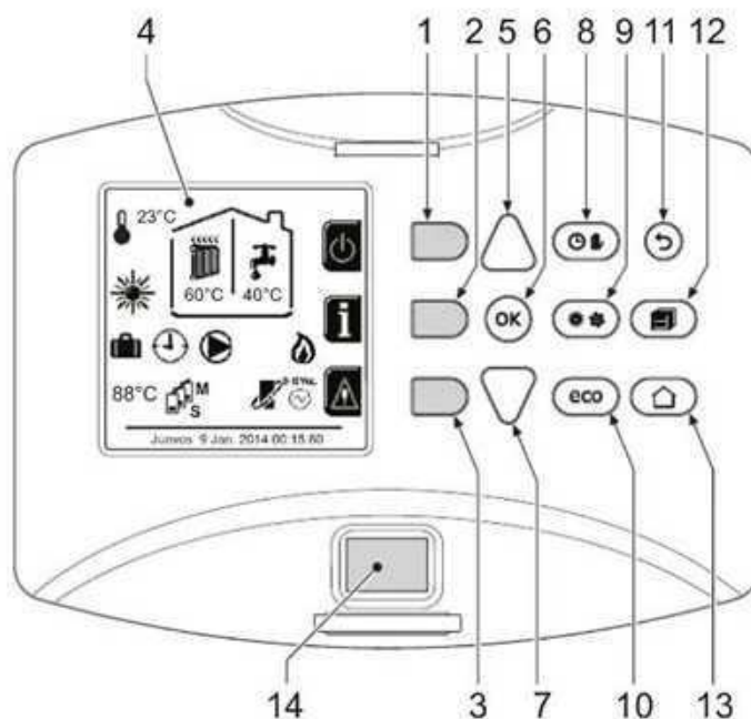
fig. 1 - Panel de control
