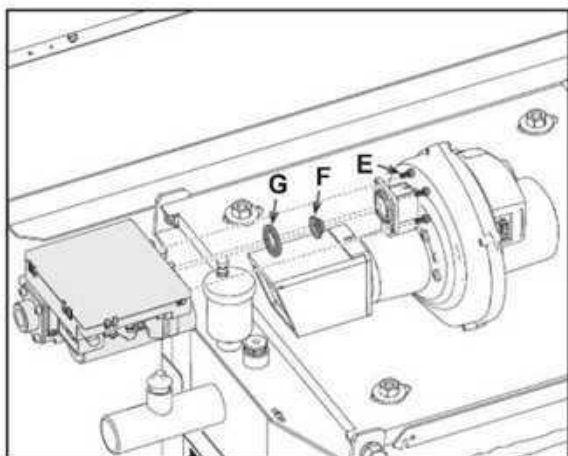
fig. 60- Model OPERA 125 and OPERA 160
