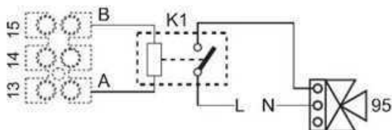
fig. 92- Connection of the 3-way valve with 2 wires
