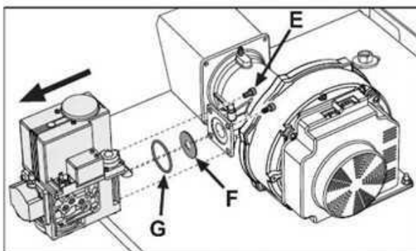
fig. 62- Model OPERA 320 and OPERA 450
