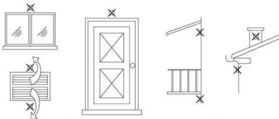
fig. 54- Positioning of external probe not recommended
