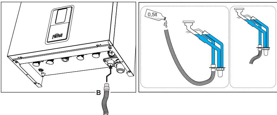
fig. 37- Condensate drain connection
