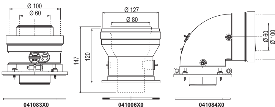
fig. 31- Starting accessories for coaxial ducts
