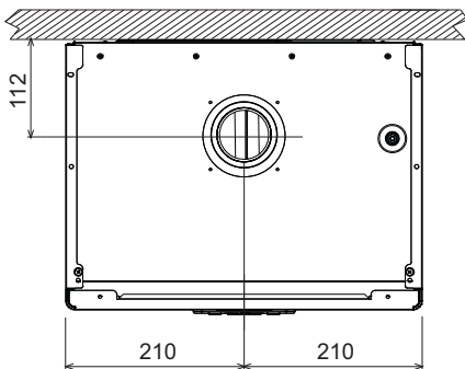
fig. 60- Top view
