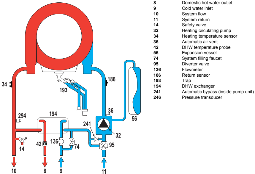
fig. 63- Hydraulic circuit
