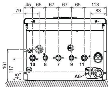
fig. 61- Bottom view
