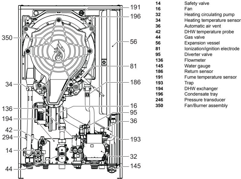
fig. 62- General view
