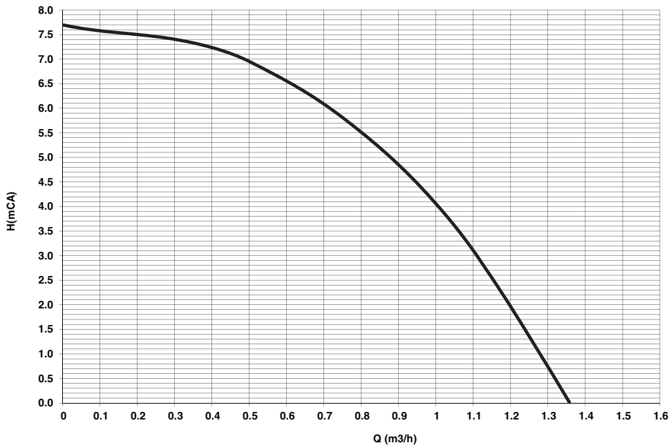
fig. 45- Residual head available for system
