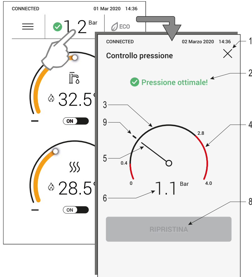
fig. 8- Pressure control
