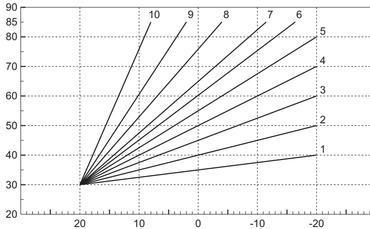
fig. 25- Compensation curves
