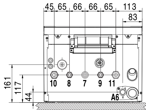
fig. 38- Bottom view
