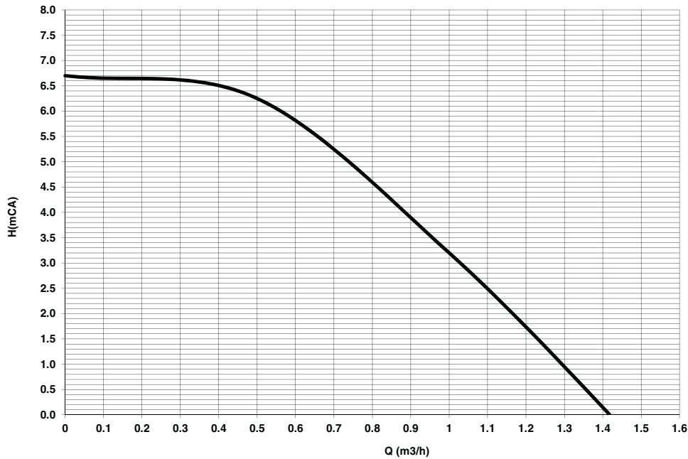
fig. 44- Residual head available for system
