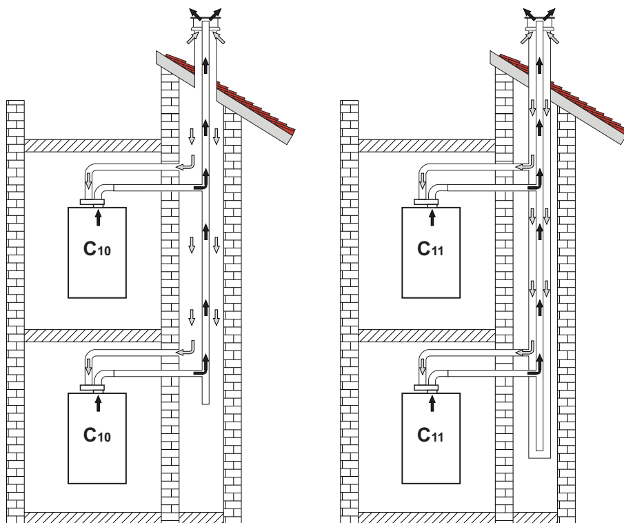
fig. 21- Connection examples - system C10 and C11 (⇐ = Air / ⇨ = Fumes)
