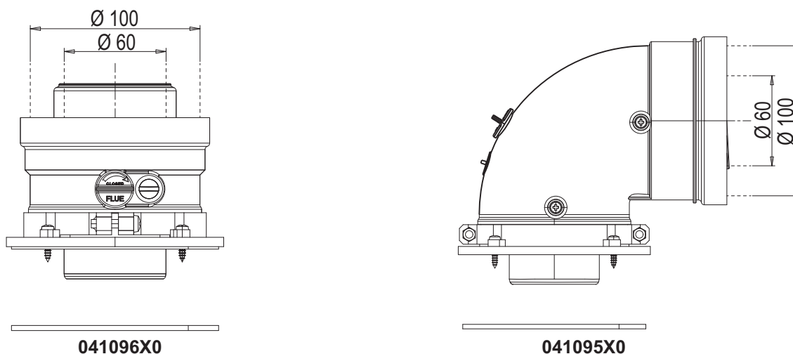
fig. 15- Starting accessories for coaxial ducts
