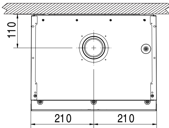
fig. 37- Top view
