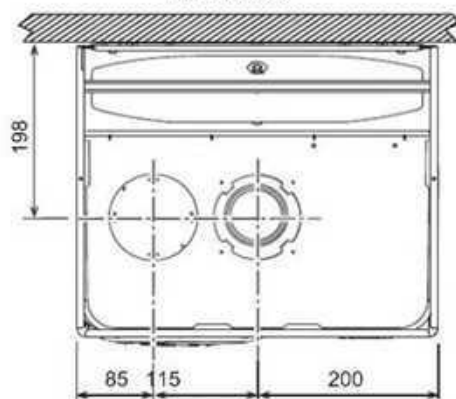
fig. 26- Top view
