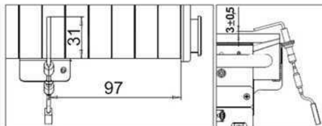
fig. 23- Electrode positioning
