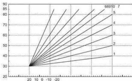
fig. 6 - Compensation curves
