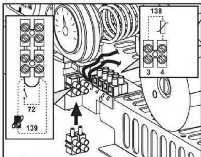
fig. 10- Accessing the terminal block
