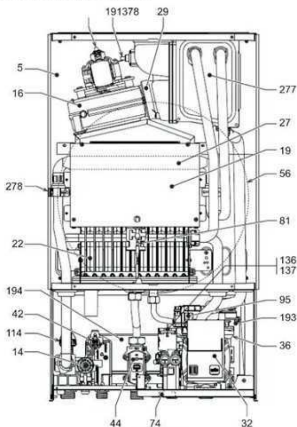
fig. 29- General view
