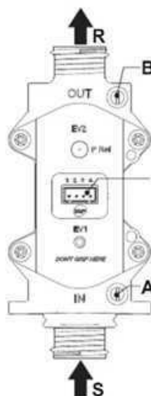
fig. 20 - Valvola gas
