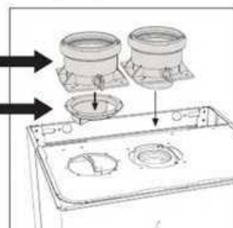
fig. 18 - Starting accessory for separate ducts
