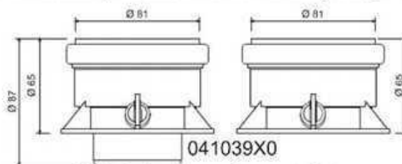
fig. 18 - Starting accessory for separate ducts
