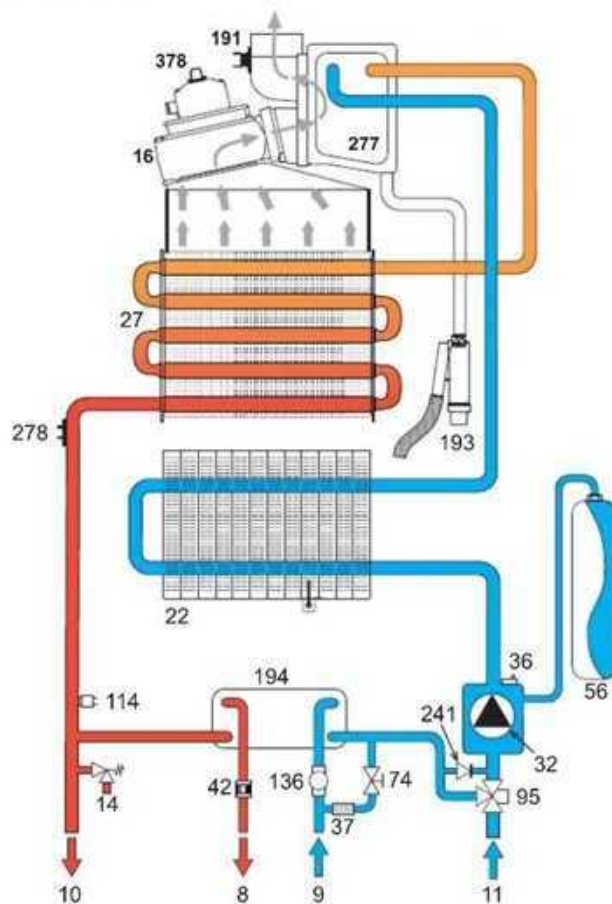
fig. 30- Heating circuit
