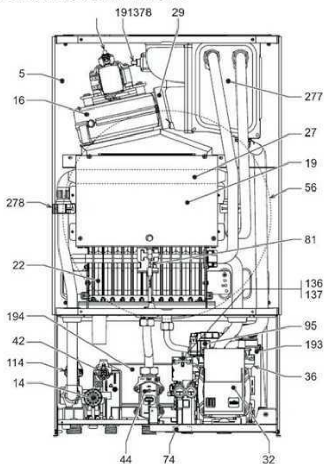
fig. 29- Vista general
