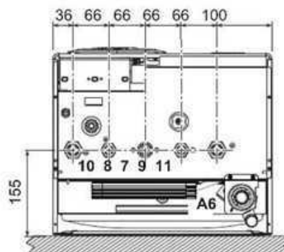
fig. 27- Bottom view
