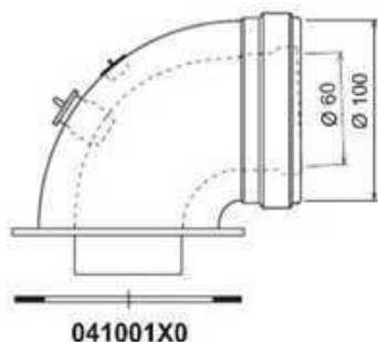
fig. 14 - Starting accessory for coaxial ducts
