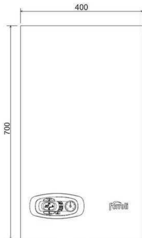
fig. 24- Front view
