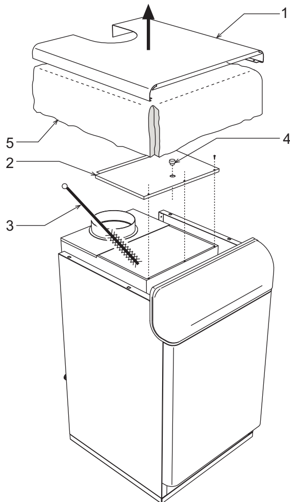
fig. 5 - Cleaning the boiler
