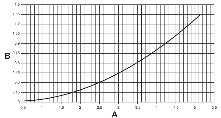
fig. 13 - Pressure losses diagram
