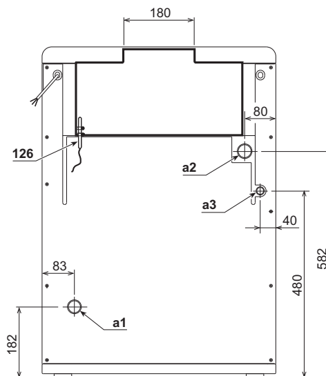
fig. 11 - Rear view
