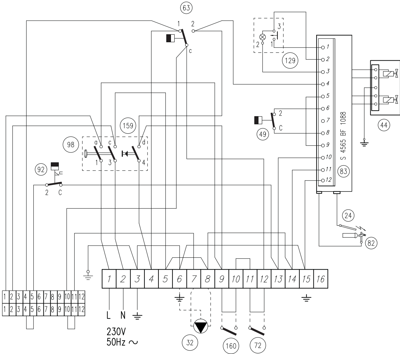
fig. 15 - Electrical connection diagram
