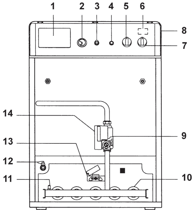
fig. 12 - General view
