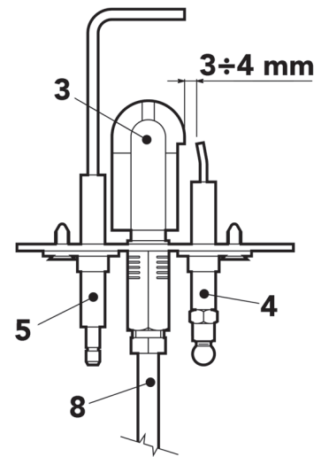
fig. 8 - Pilot burner
