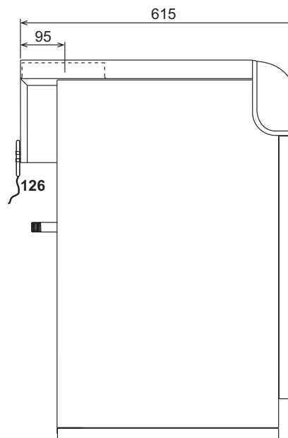
fig. 10 - Side view
