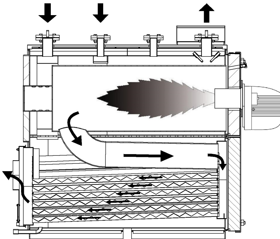
fig. 1 - Working principle
