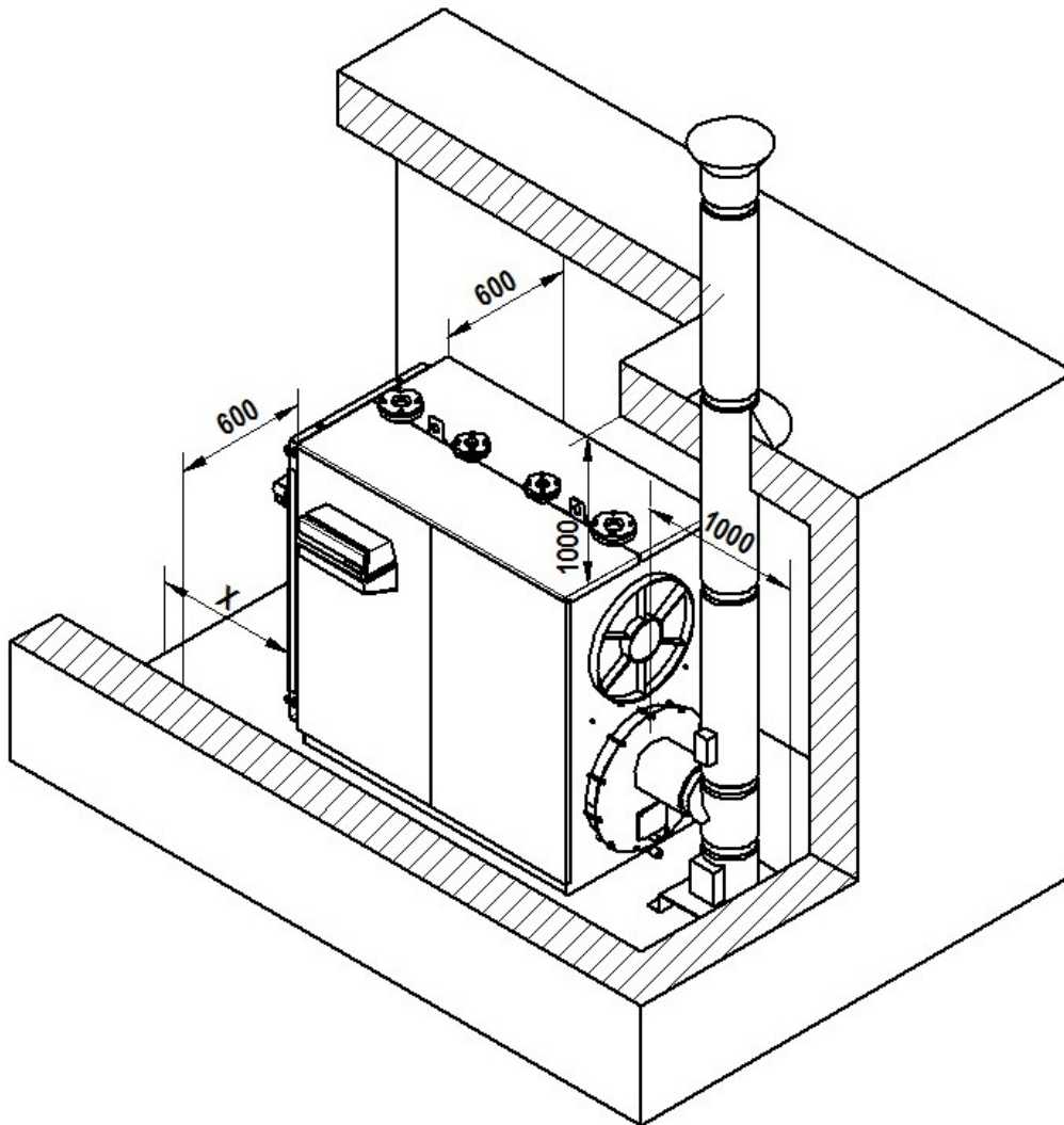
fig. 6 - Installation room
