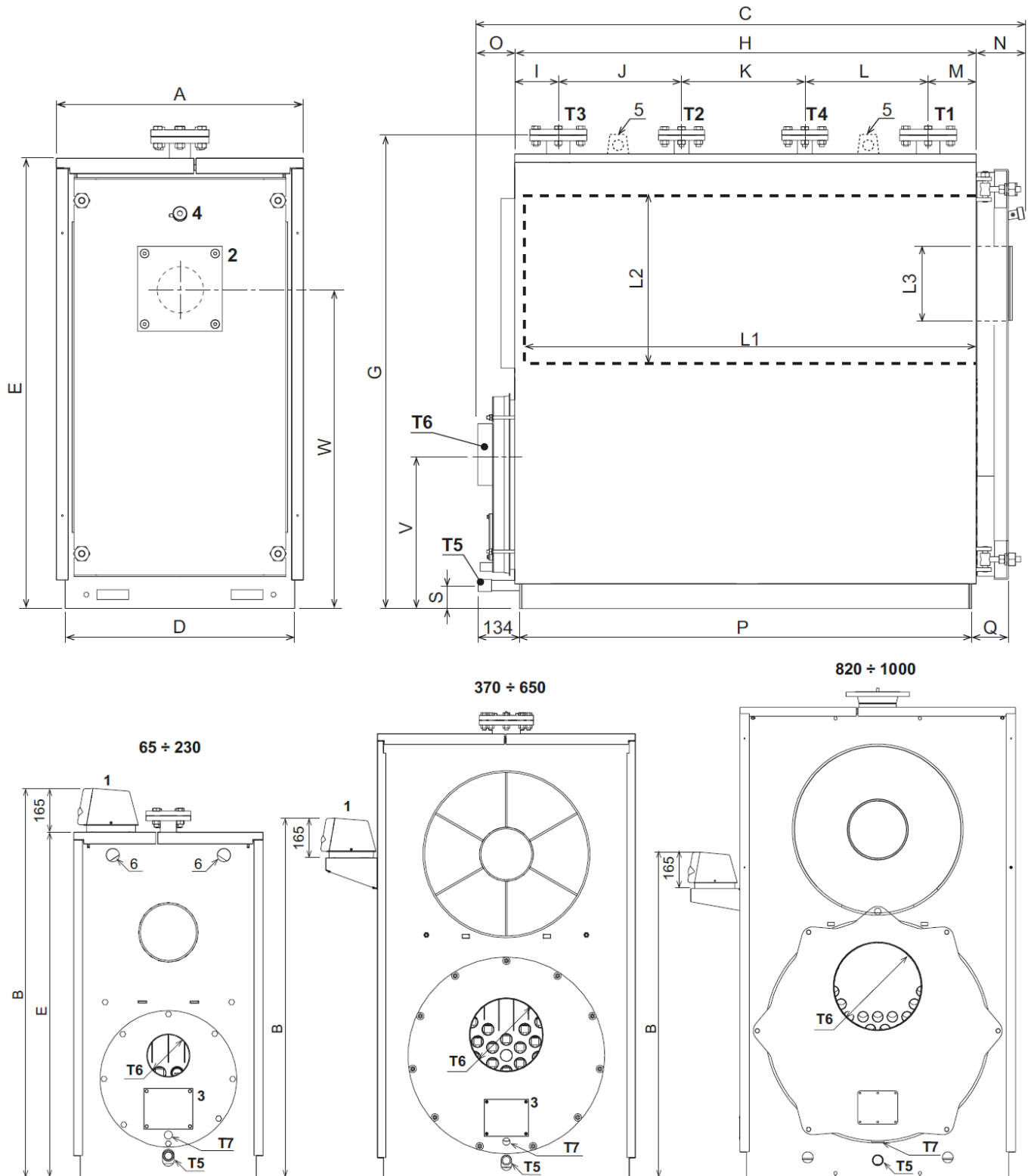
fig. 2 - Dimensions and connections
