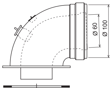
041001X0 fig. 17 - Starting accessory for coaxial ducts
