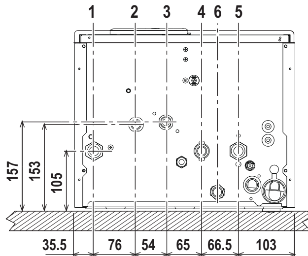
fig. 13 - Plumbing connections
