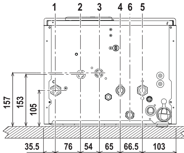
fig. 13 - Raccordements hydrauliques
