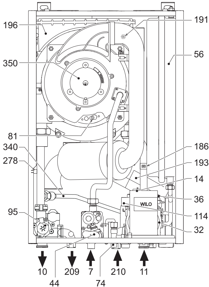
fig. 27 - General view
