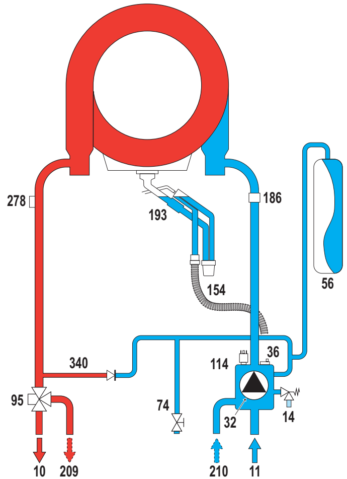
fig. 28 - Water circuit
