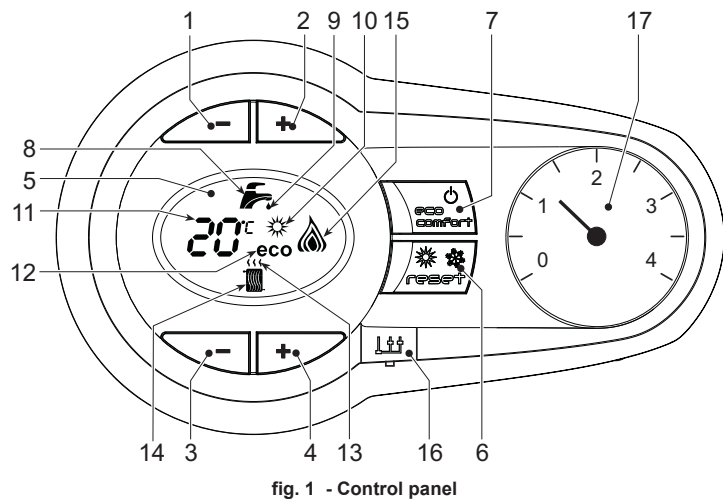
fig. 1 - Control panel
