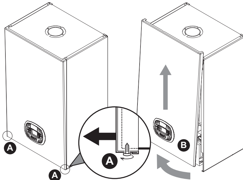
fig. 32- Front panel opening
