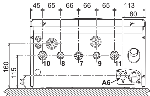
fig. 56- Bottom view
