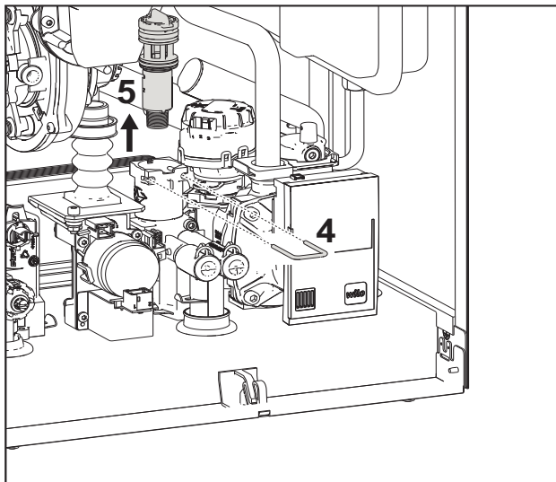
fig. 47- Flowmeter
