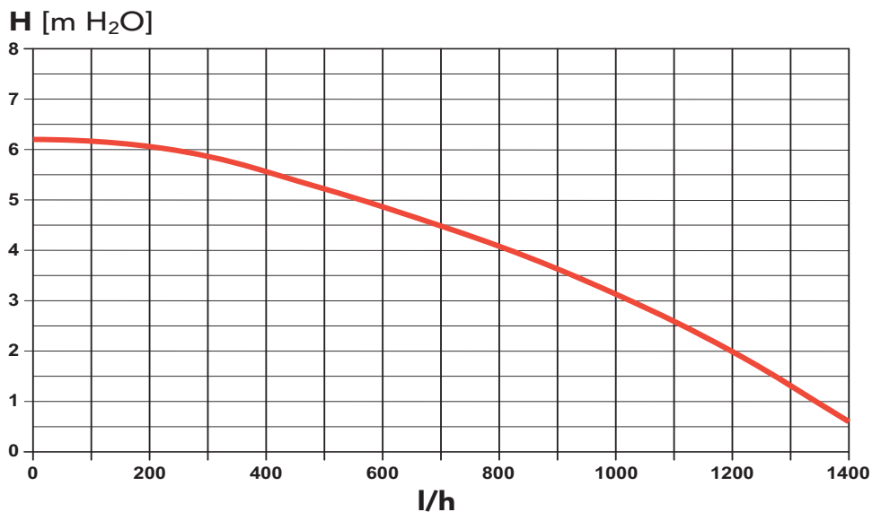
fig. 61- Residual head available for system
