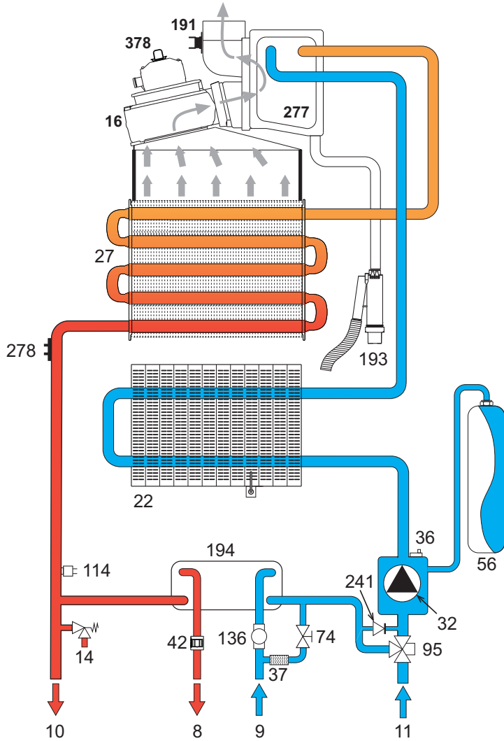
fig. 27- Heating circuit
