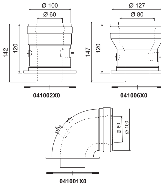
fig. 13 - Starting accessory for coaxial ducts
