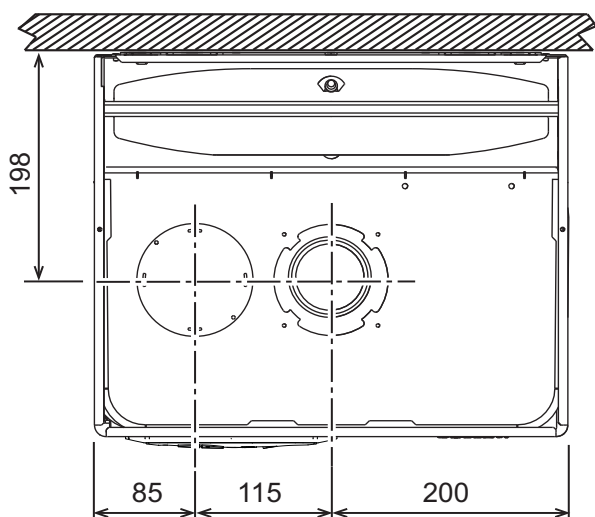
fig. 23- Top view
