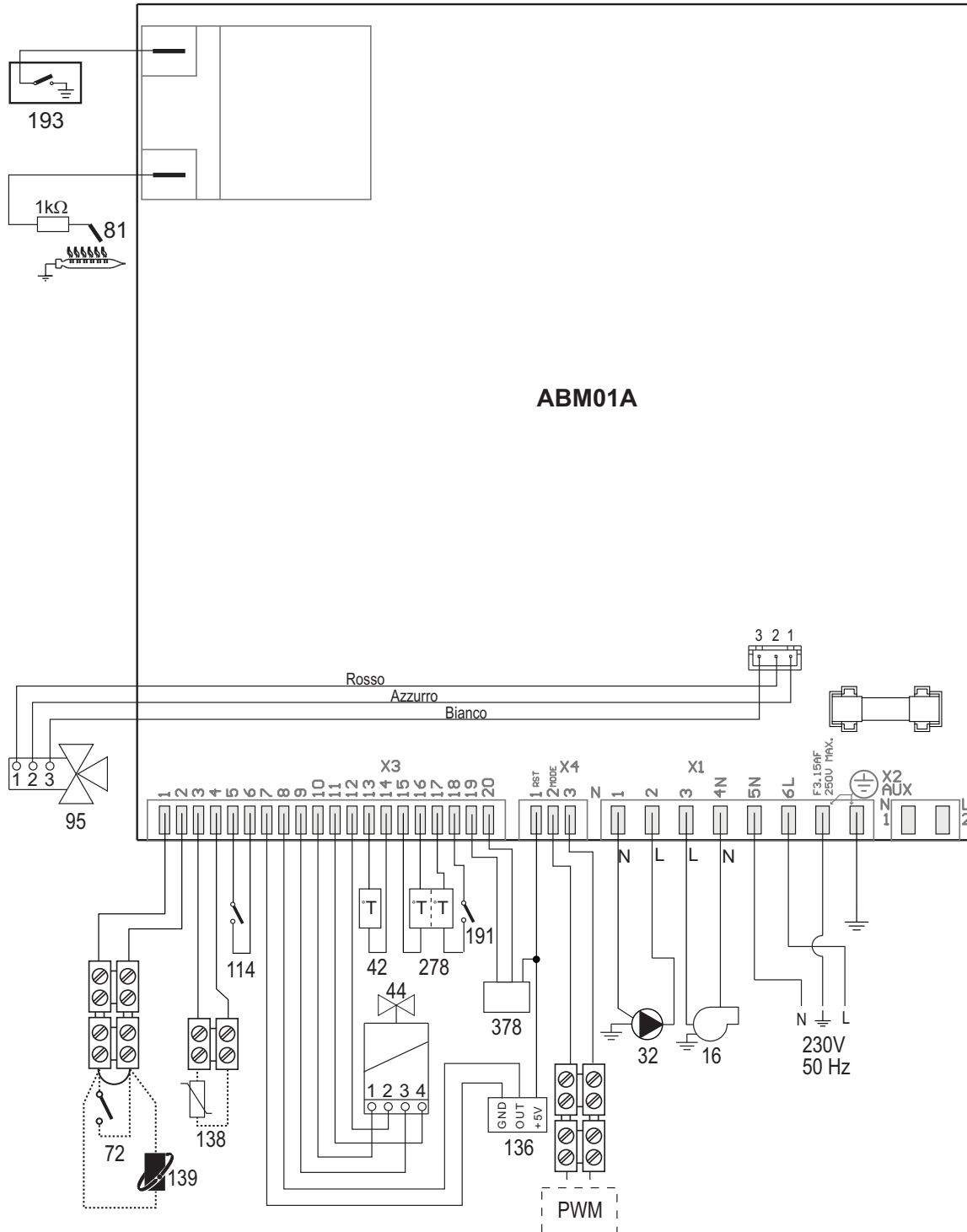
fig. 28- Wiring diagram
