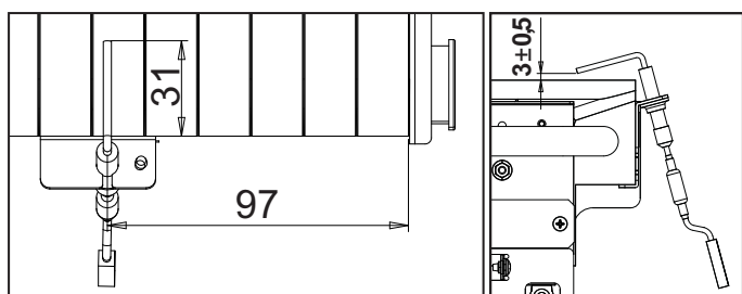
fig. 20- Electrode positioning
