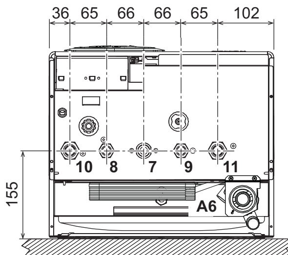
fig. 24- Bottom view
