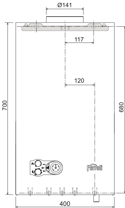
fig. 8 - Front view
