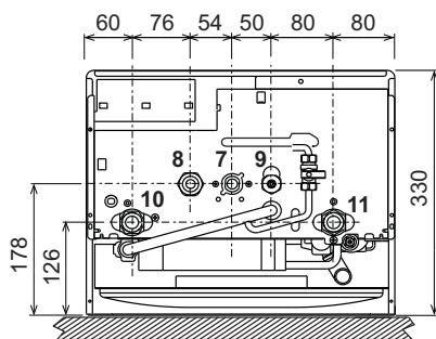
fig. 10 - Bottom view
