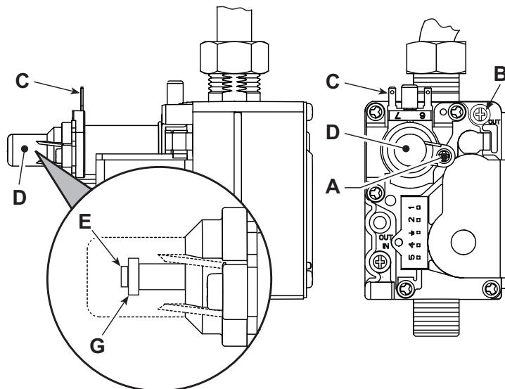
fig. 6 - Gas valve
