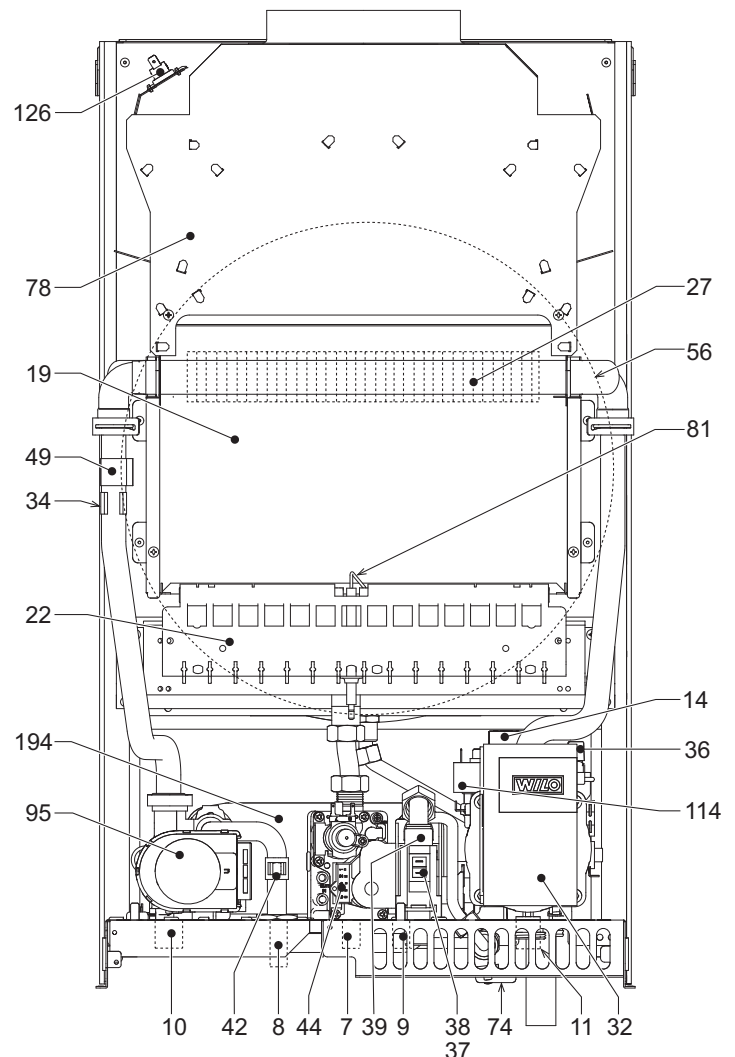
fig. 12 - General view
