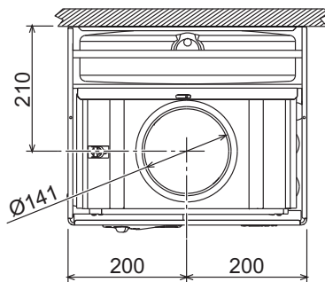
fig. 9 - Top view
