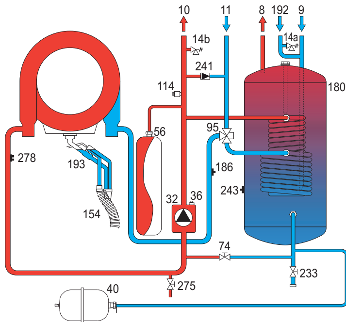
fig. 29 - Water circuit
