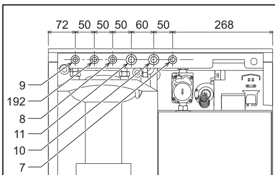
fig. 13 - Raccordements hydrauliques
