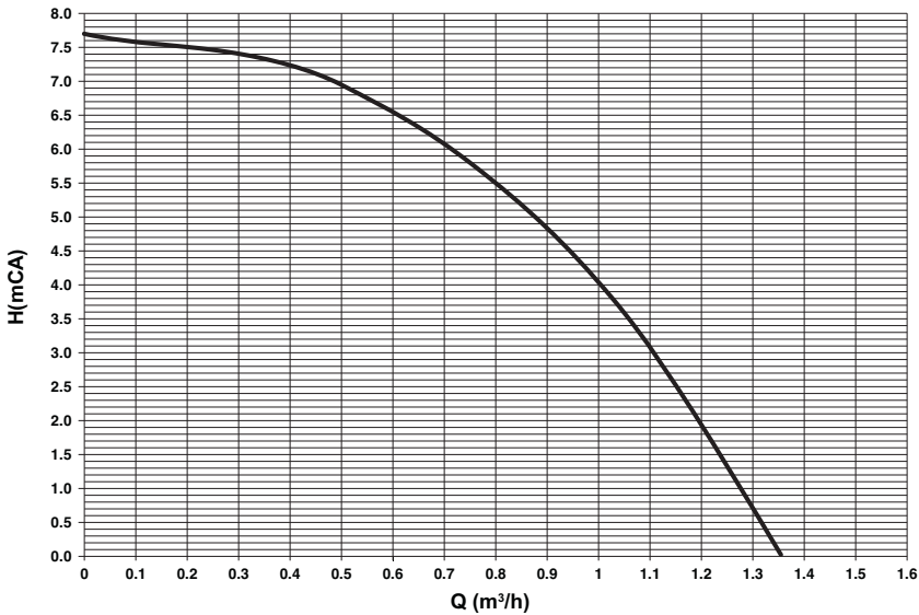
fig. 79- Residual head available for system
