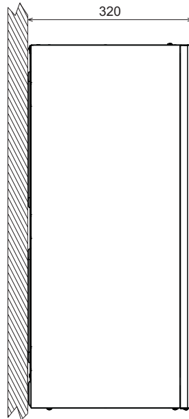
fig. 73- Side view
