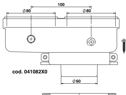
fig. 36- Starting accessory for separate ducts
