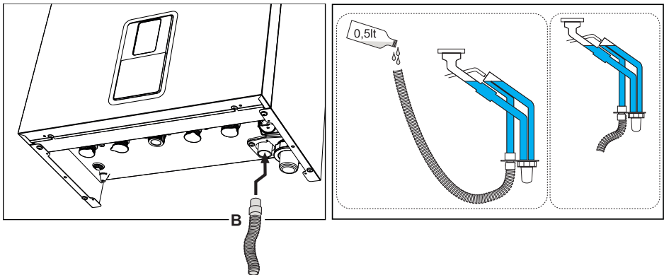
fig. 52- Condensate drain connection
