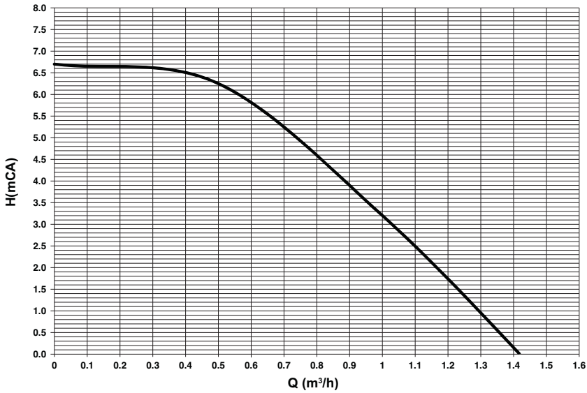
fig. 78- Residual head available for system
