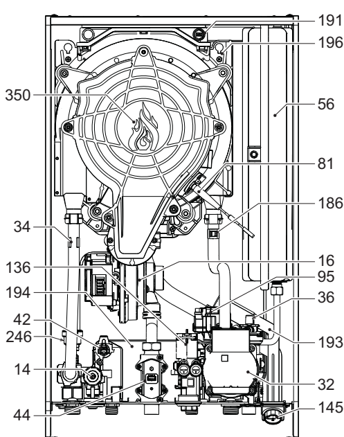
fig. 76- General view
