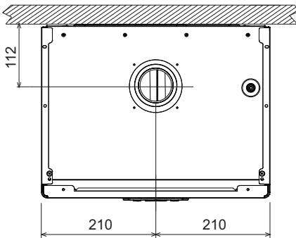
fig. 74- Top view
