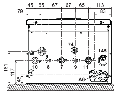
fig. 75- Bottom view
