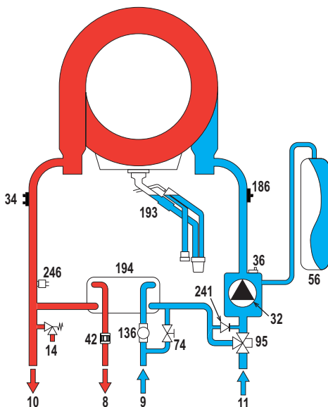
fig. 77- Hydraulic circuit
