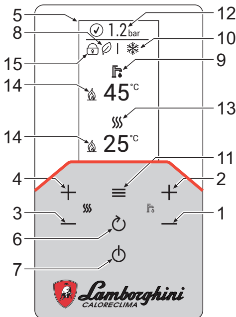
fig. 1- Control panel
