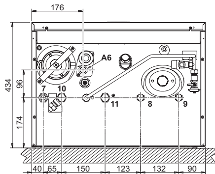
fig. 46- Bottom view
