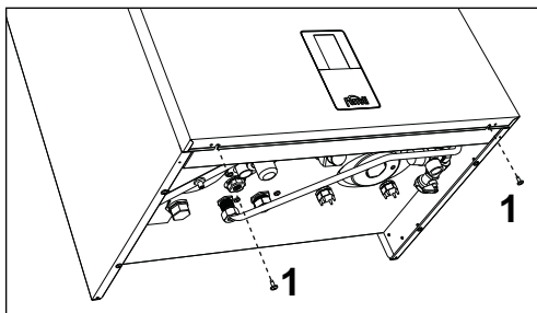
fig. 41- Front panel opening
