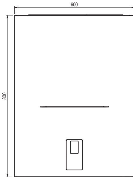
fig. 43- Front view
