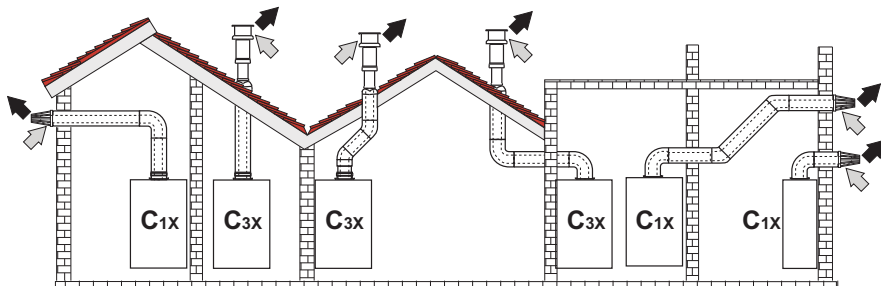
fig. 30- Examples of connection with coaxial pipes (⇐ = Air / ⇨ = Fumes)
