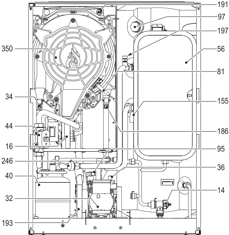
fig. 47- General view
