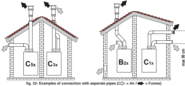
fig. 32- Examples of connection with separate pipes (↔ = Air / ↗ = Fumes)
