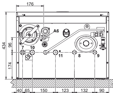
fig. 46- Bottom view
