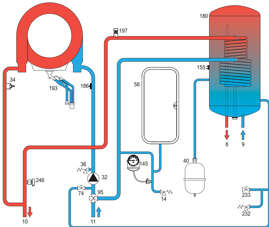
fig. 48- Hydraulic circuit
