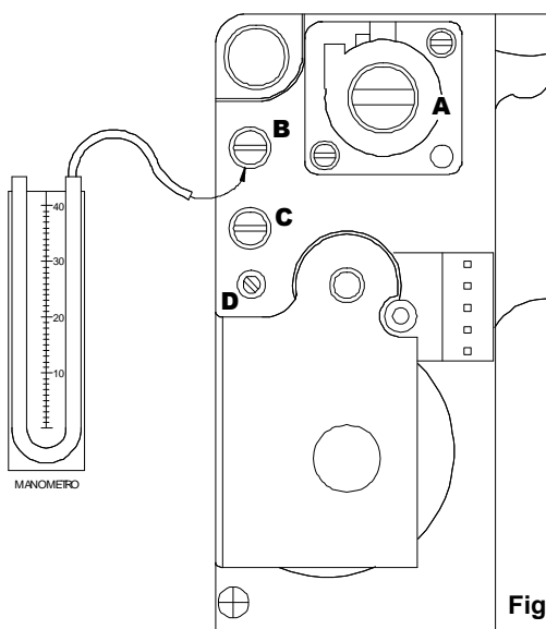
Valvola gas VK 4105G
