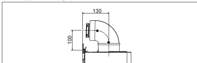
Conducte ramificate Ø 80 mm
