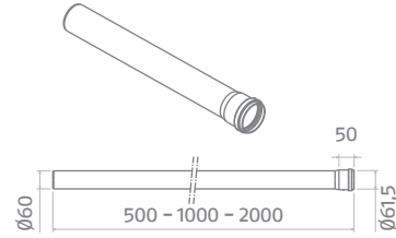
Prolunga \varnothing 60 mm (500-1000-2000 mm)
