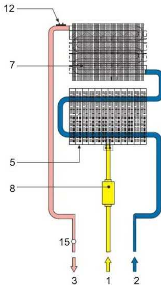
fig. 25 - Hydraulic circuit
