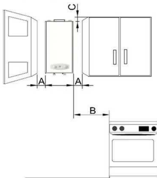
fig. 5 - Minimum distances
