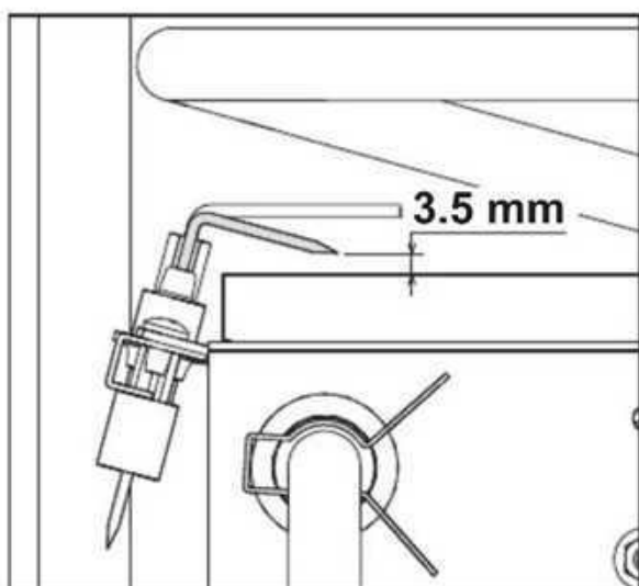
fig. 16 - Electrode position
