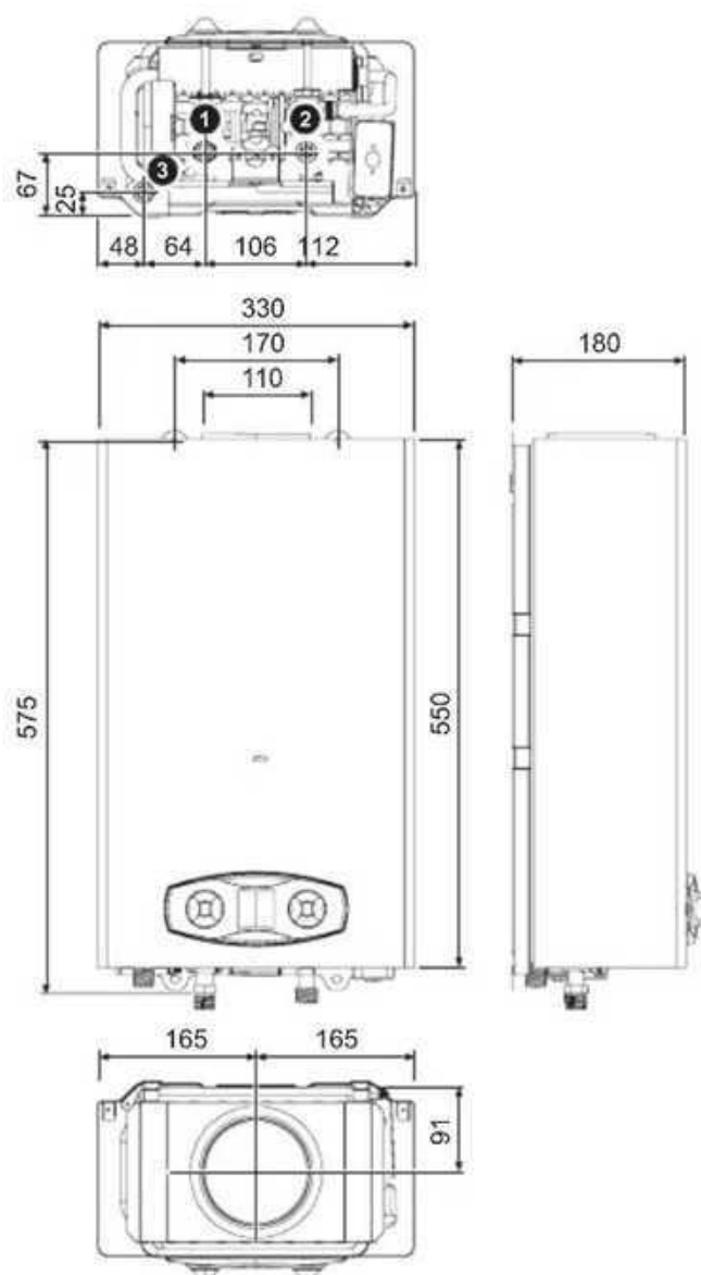
fig. 20 - Dimensions and connections ZEFIRO ECO 11
