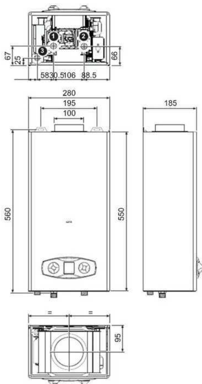
fig. 19 - Dimensions and connections ZEFIRO ECO 6
